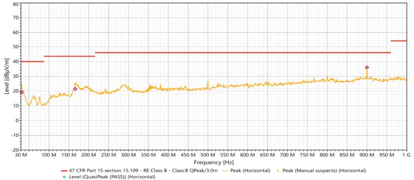
#2 - 30MHz-1GHz (Horizontal)
