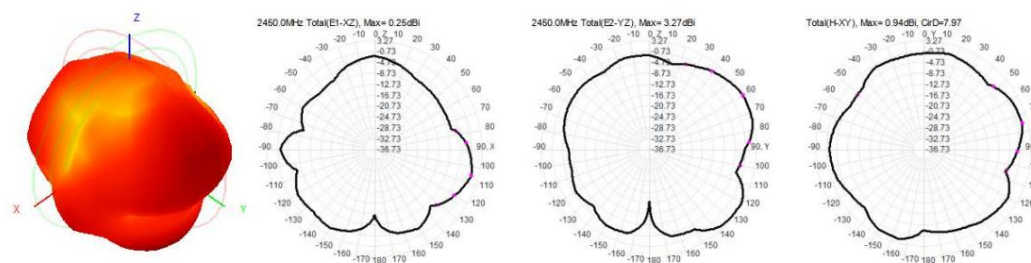
WiFi Location 1-2450MHz
