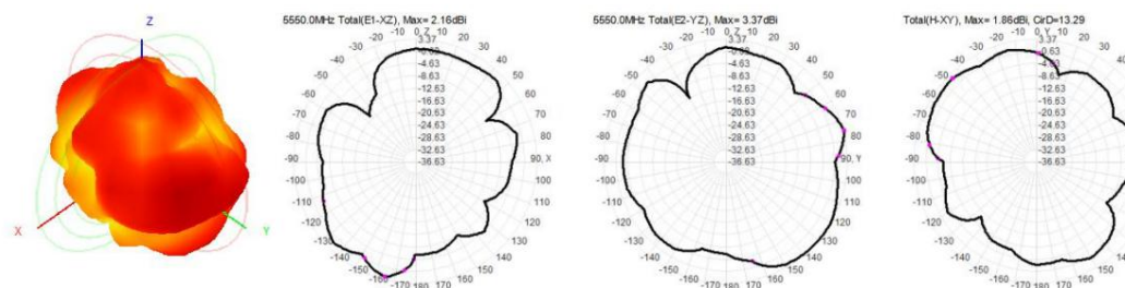
WiFi location 2-5550MHz
