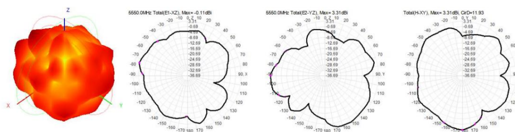
WiFi Location 1-5550MHz
