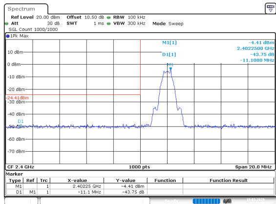
BLE_1M_Low_Channel
