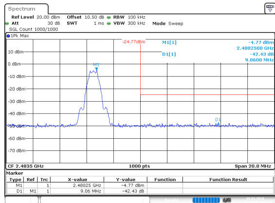
BLE_1M_High_Channel
