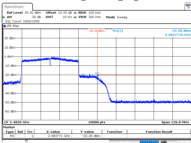
802.11ax40_2452MHz_RU_Full
