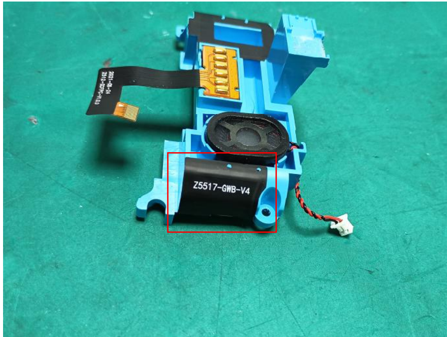
BT/Wi-Fi ANT
