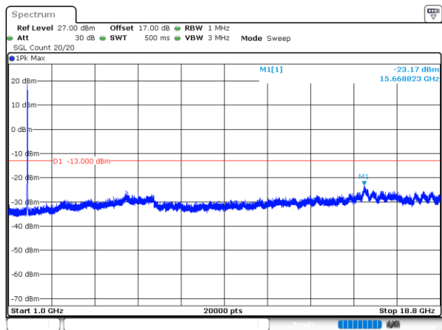
15MHz_High_QPSK_75@0(1GHz~18.8GHz)
