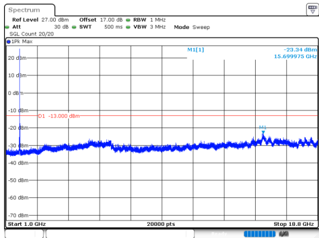
15MHz_High_QPSK_1@0(1GHz~18.8GHz)
