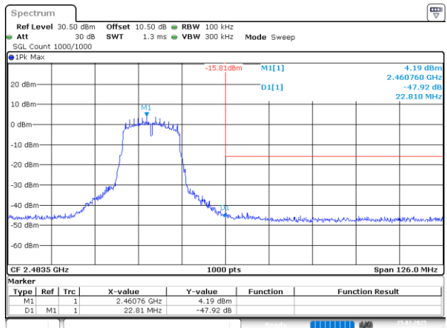
802.11g_2462MHz
