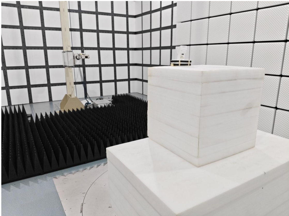
Radiated Spurious Emissions Test View (18GHz-40GHz)
