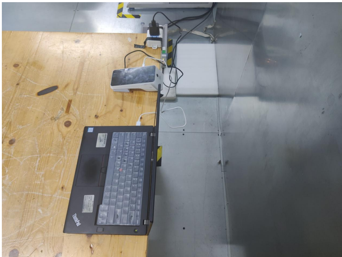
Photo of Power Line Conducted Emission Measurement-Side View(Test Mode 4)
