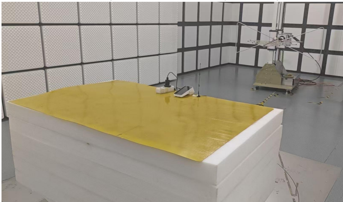
Radiated Spurious Emissions Test View (30MHz- 1GHz)
