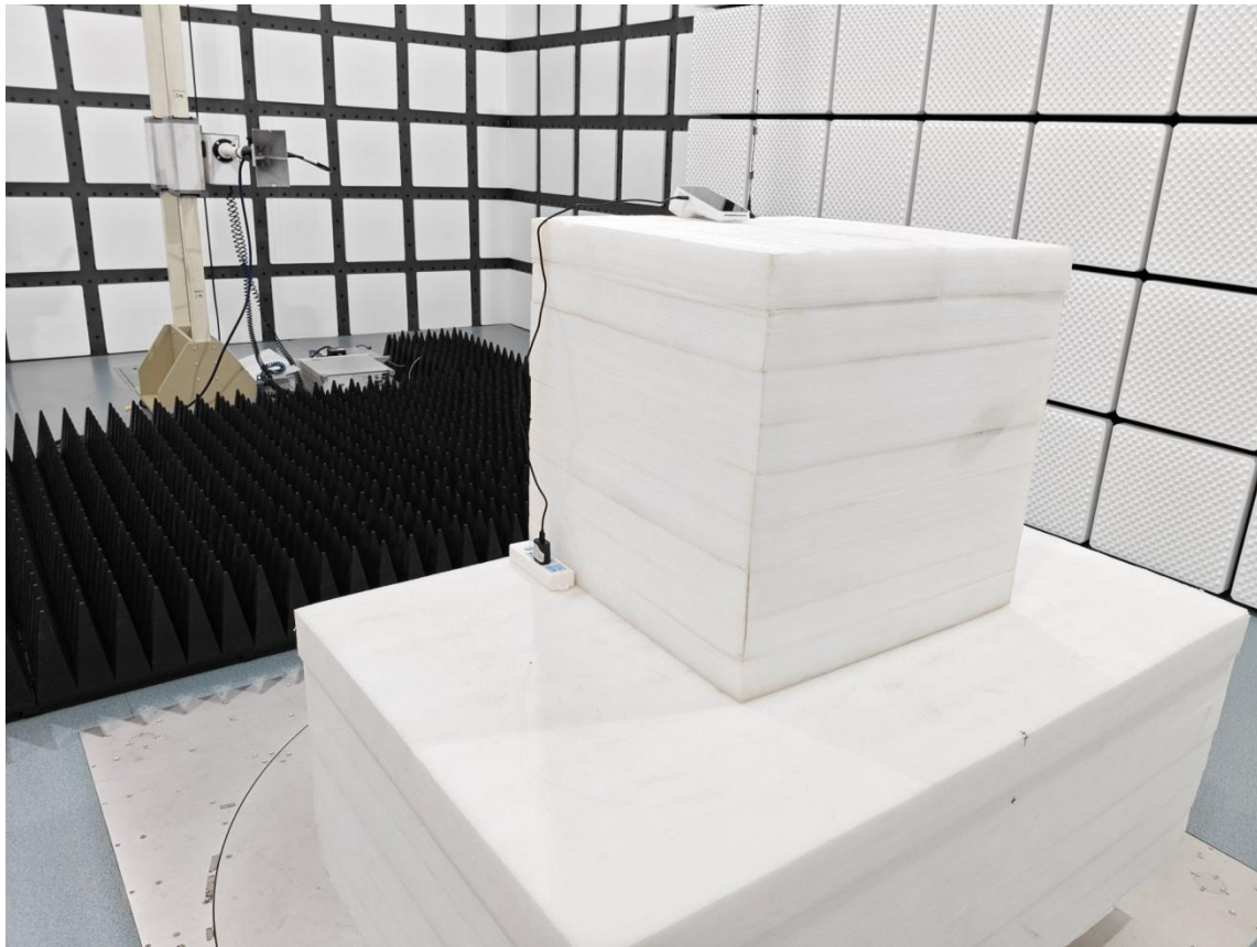
Radiated Spurious Emissions Test View (Above 1GHz)
