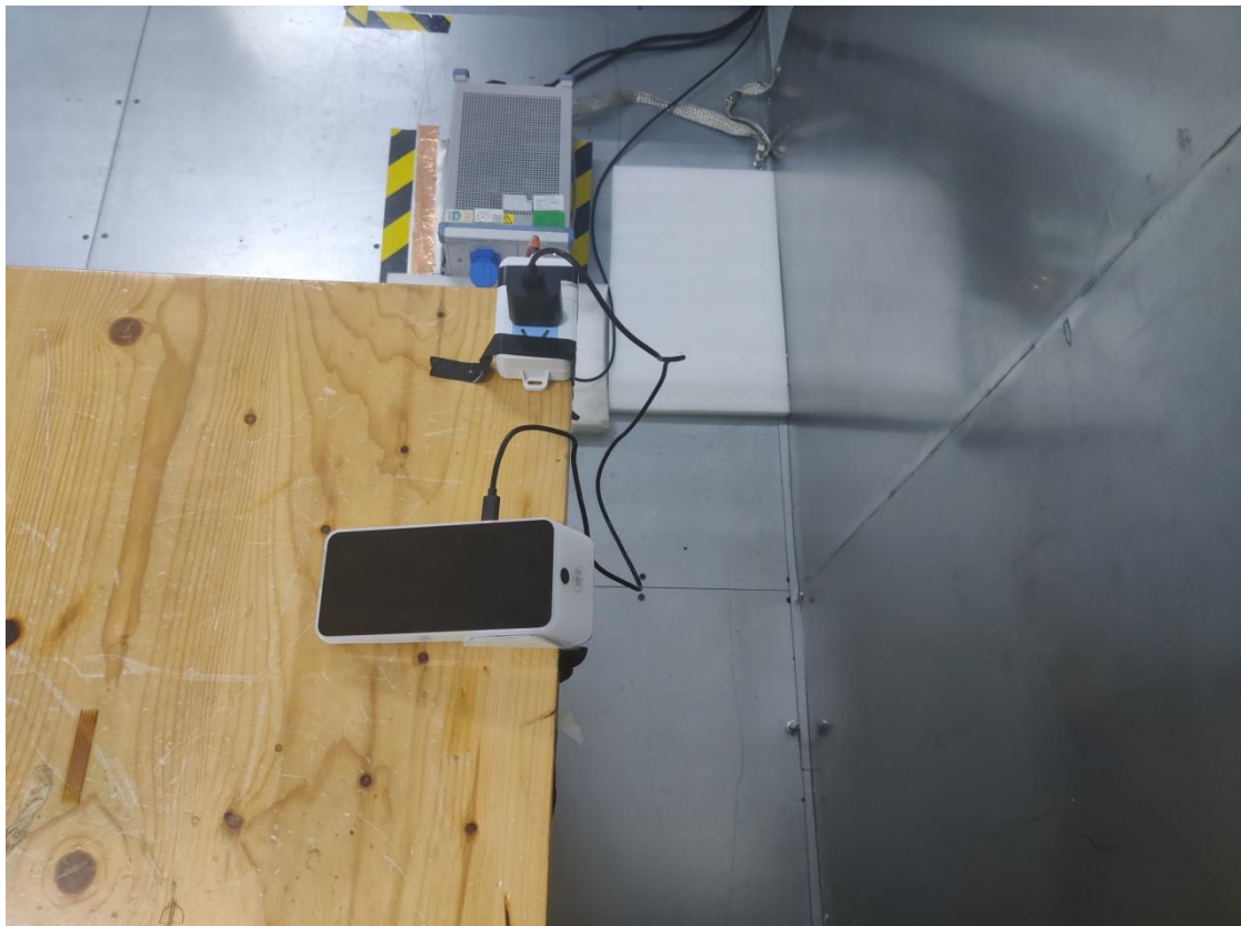
Photo of Power Line Conducted Emission Measurement-Side View(Test Mode 1&2)
