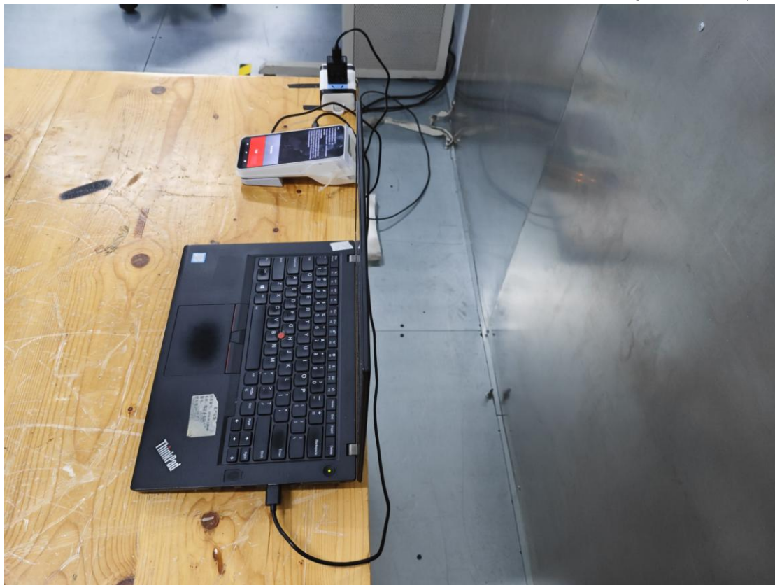
Photo of Power Line Conducted Emission Measurement-Front View(Test Mode 4)
