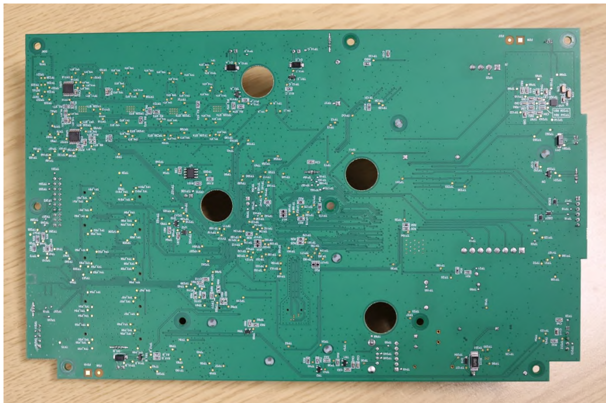
Control_PCBA_Bottom
