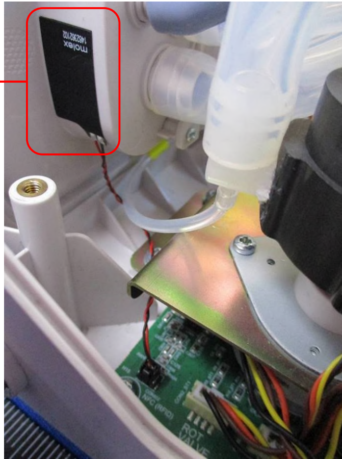
13.56 MHz Antenna
