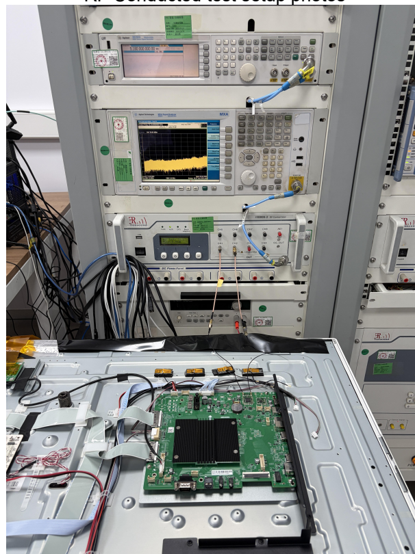
RF Conducted test setup photos
