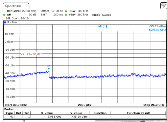
BLE_1M_Low_Channel
