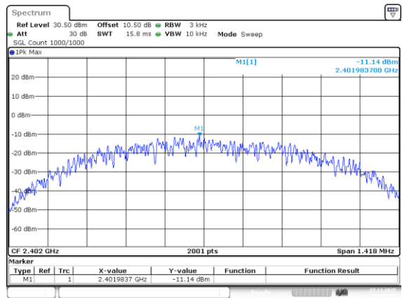
BLE_1M_Low_Channel
