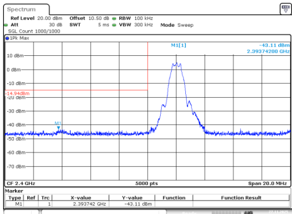
BLE_1M_Low_Channel
