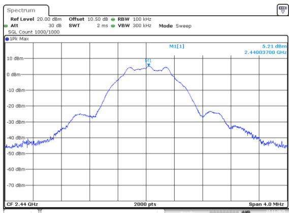
BLE_1M_Middle_Channel
