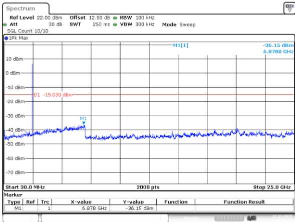
BLE_1M_High_Channel
