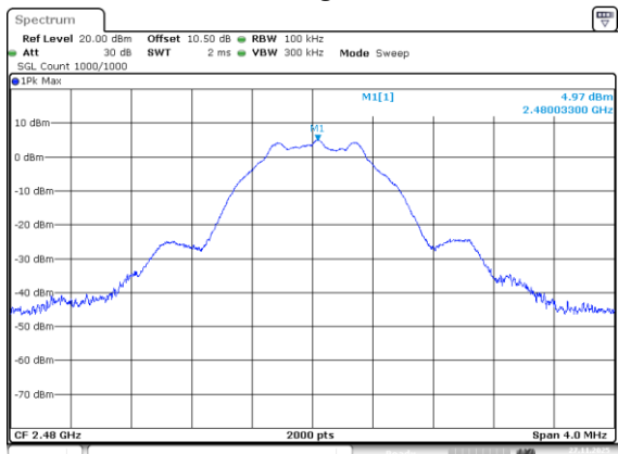
BLE_1M_High_Channel
