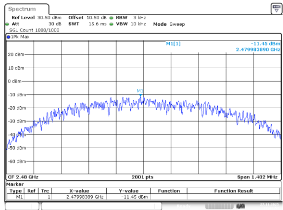
BLE_1M_High_Channel
