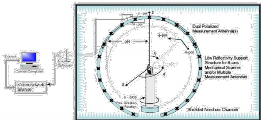
测试系统Test System
