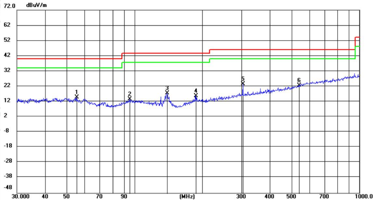
Test Graph of Horizontal:
