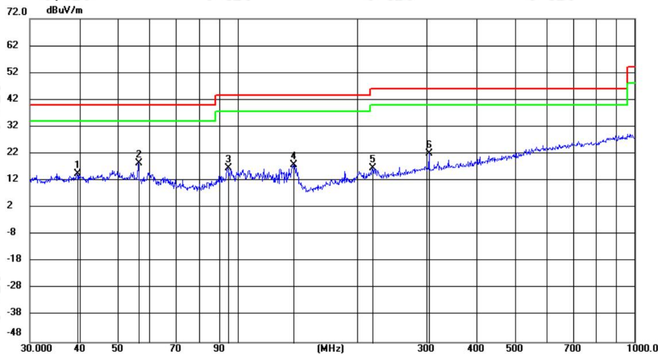
Test Graph of Vertical:
