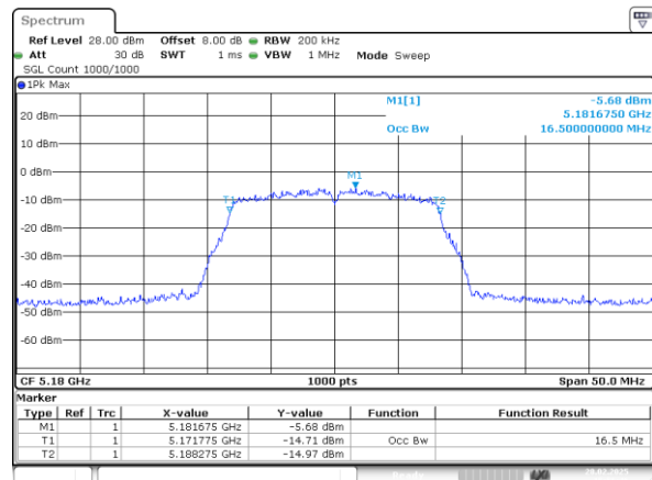
802.11a_5180MHz_Chain 1
