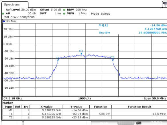
802.11a_5180MHz_Chain 0
