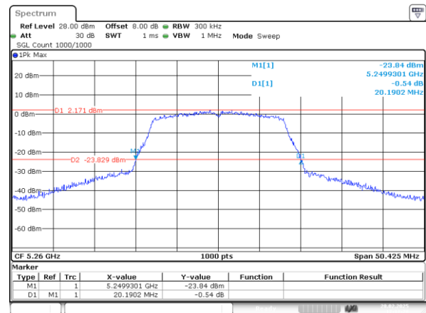
802.11a_5260MHz_Chain 1
