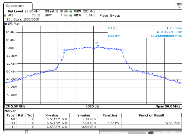
802.11a_5580MHz_Chain 1
