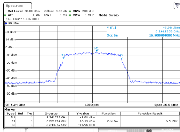
802.11a_5240MHz_Chain 1
