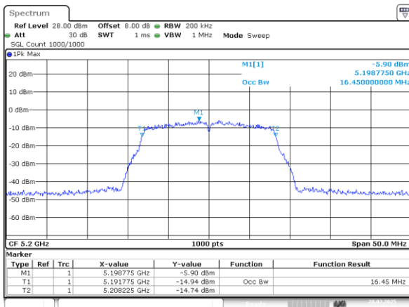
802.11a_5200MHz_Chain 1
