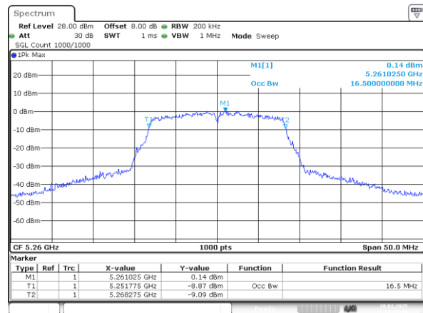
802.11a_5260MHz_Chain 1
