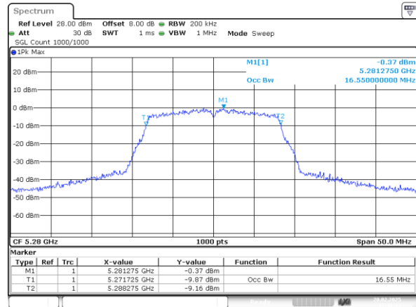
802.11a_5280MHz_Chain 0
