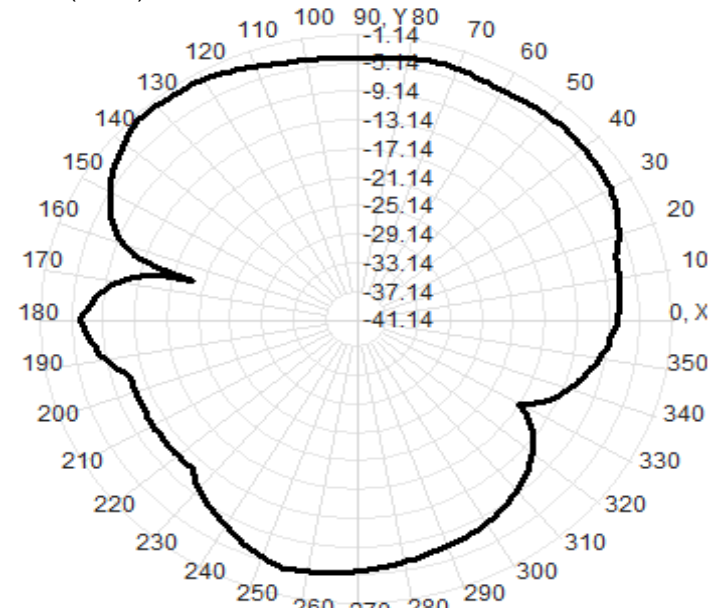
Total(H-XY), Max=-1.93dB, CirD=17.90
