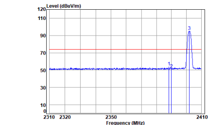
BLE_1M_TX_CH_00_Vertical-Peak
