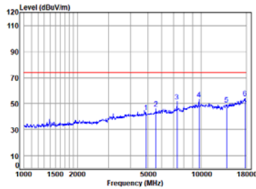
BLE_1M_TX_CH_19_Vertical-Peak
