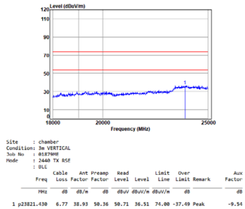
BLE_1M_TX_CH_19_Vertical-Peak
