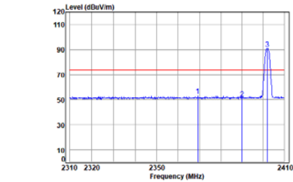
BLE_1M_TX_CH_00_Horizontal-Peak
