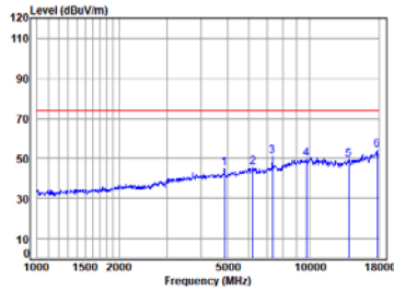
BLE_1M_TX_CH_19_Horizontal-Peak
