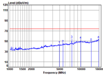
BLE_1M_TX_CH_39_Vertical-Peak
