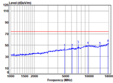
BLE_2M_TX_CH_19_Horizontal-Peak
