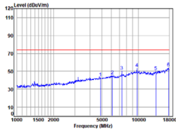
BLE_2M_TX_CH_19_Vertical-Peak
