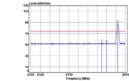
BLE_1M_TX_CH_00_Vertical-Peak
