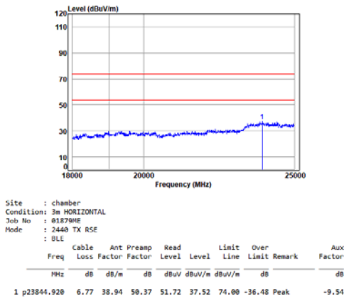
BLE_1M_TX_CH_19_Horizontal-Peak
