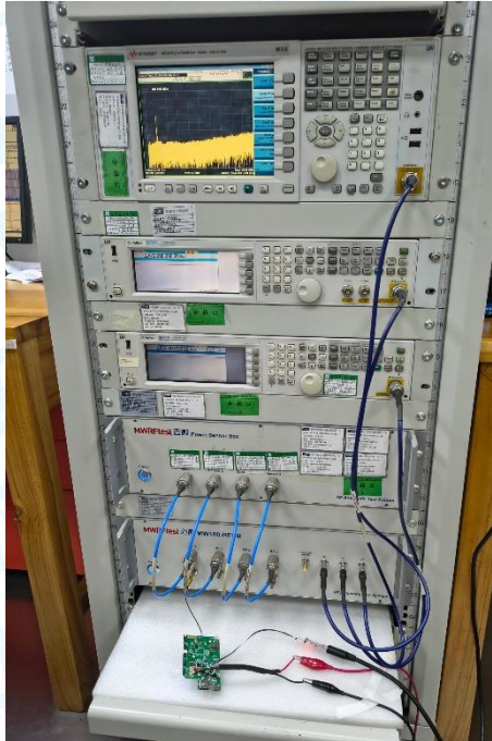
Photo of Setup for Conducted Measurement
