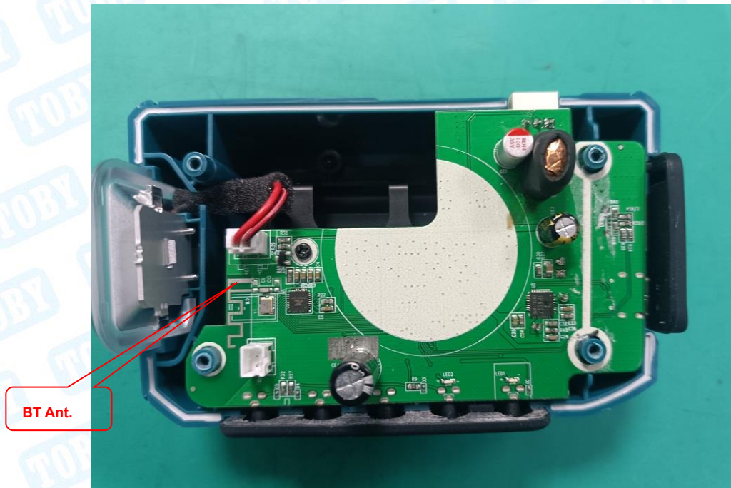
Photo 14 Appearance of PCB
