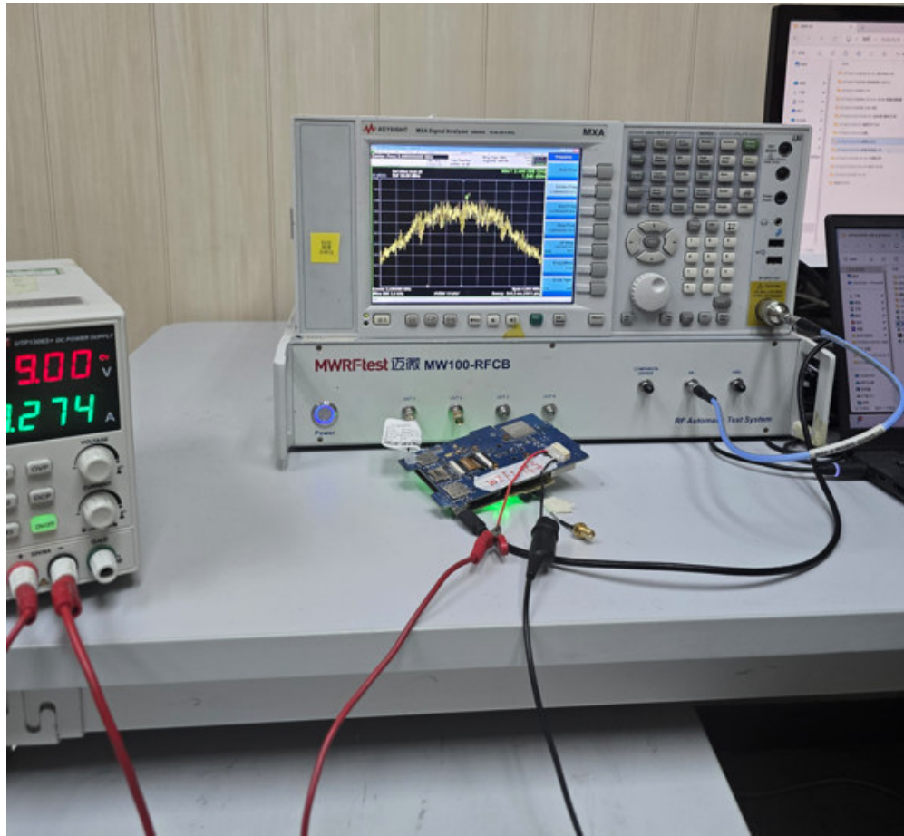
Wi-Fi 2.4GHz Test Setup
