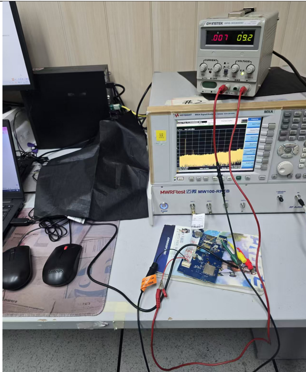
Bluetooth LE Test Setup
