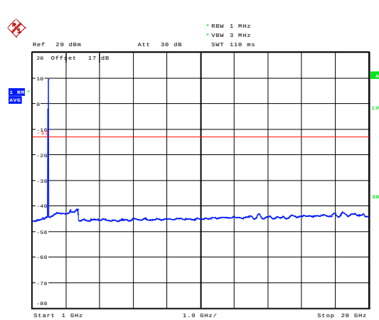
LTE Band 25 1.4MHz CH-Middle 1GHz~20GHz
