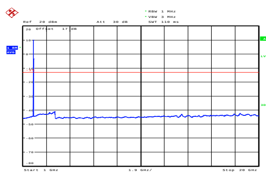
LTE Band 25 1.4MHz CH-Low 1GHz~20GHz
