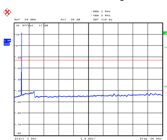
LTE Band 25 1.4MHz CH-High 1GHz~20GHz
