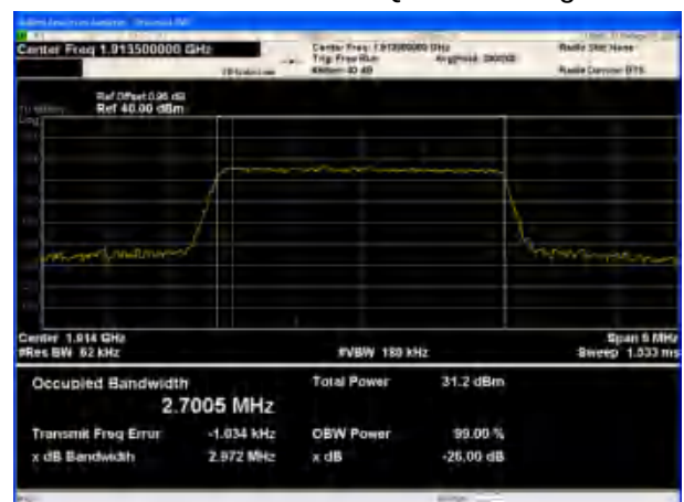
LTE Band 25 3MHz QPSK CH-High
