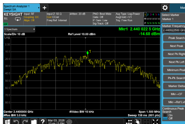
GFSK (BLE 1Mbps) MIDDLE CHANNEL
