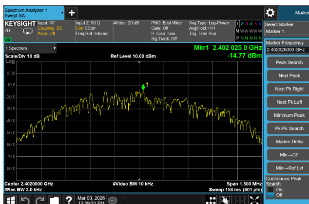
GFSK (BLE 1Mbps) LOW CHANNEL
