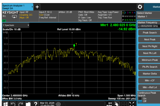
GFSK (BLE 1Mbps) HIGH CHANNEL
