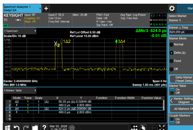
GFSK (BLE 2Mbps)
