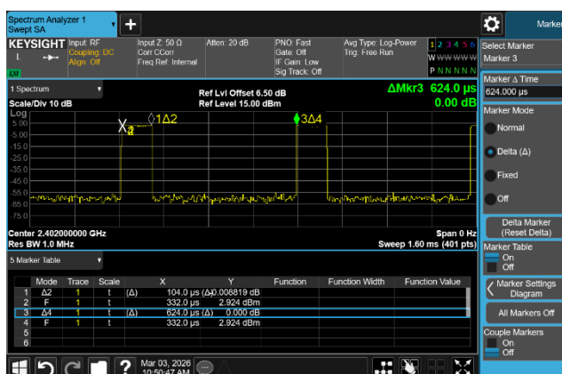
GFSK (BLE 1Mbps)
