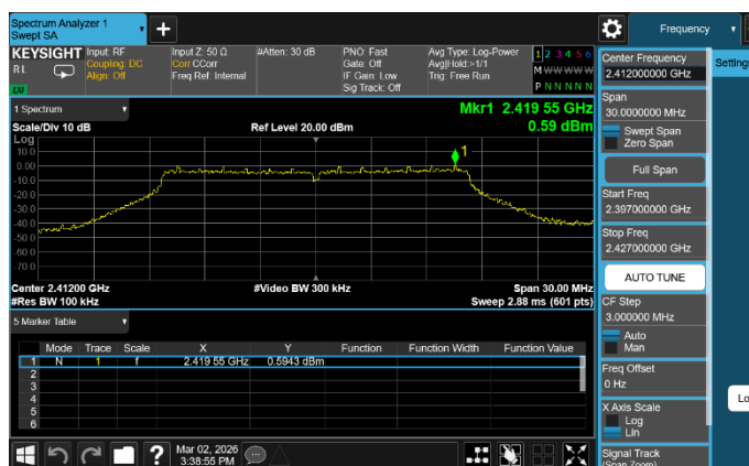
802.11g LOW CHANNEL, CARRIER LEVEL
