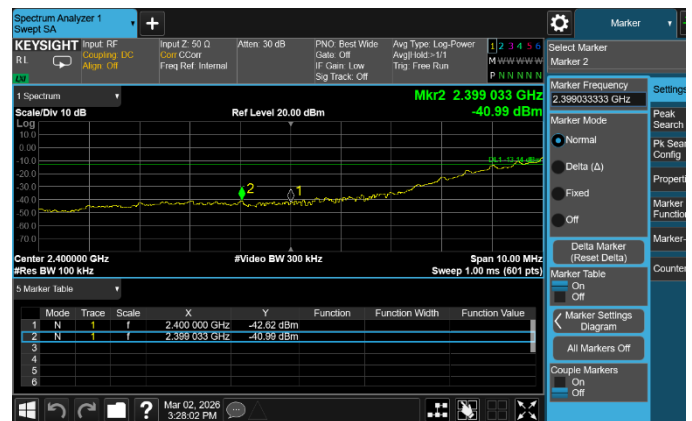
802.11b LOW CHANNEL, BAND EDGE
