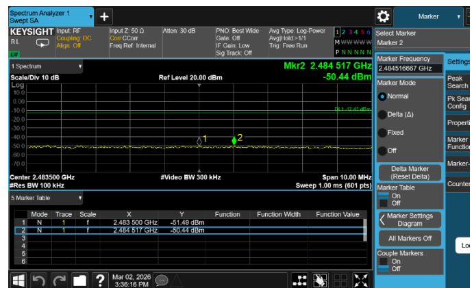
802.11b HIGH CHANNEL, BAND EDGE
