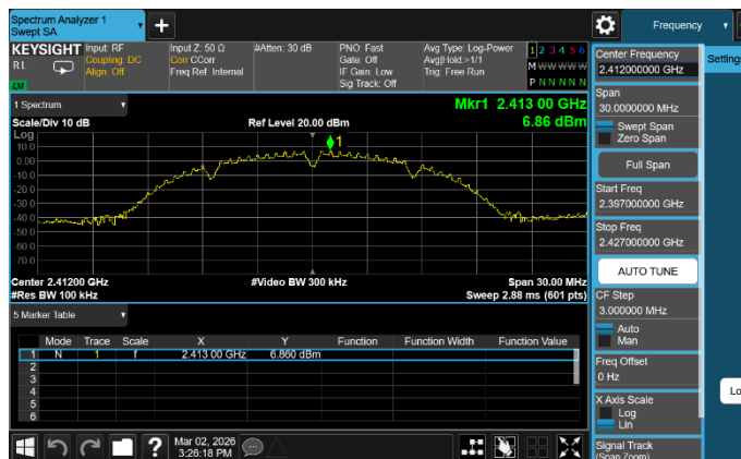
802.11b LOW CHANNEL, CARRIER LEVEL
