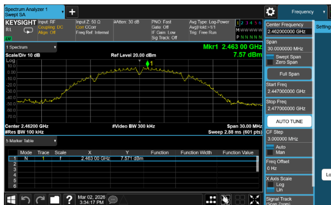
802.11b HIGH CHANNEL, CARRIER LEVEL
