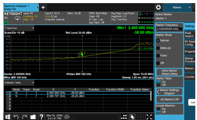
802.11g LOW CHANNEL, BAND EDGE
