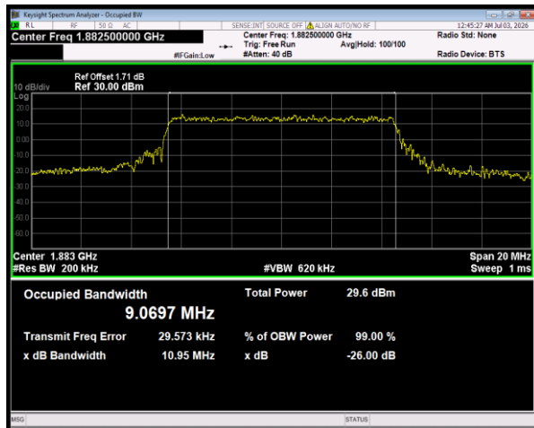
Band25 QPSK BW=10MHz Channel=26365 RB Size=50 Position=#0
