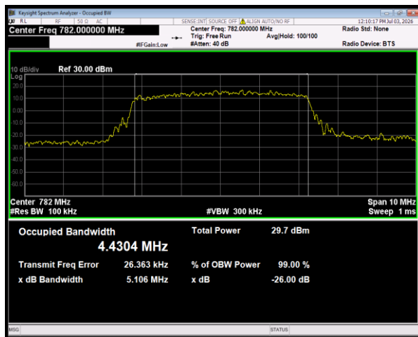
Band13 QPSK BW=5MHz Channel=23230 RB Size=25 Position=#0
