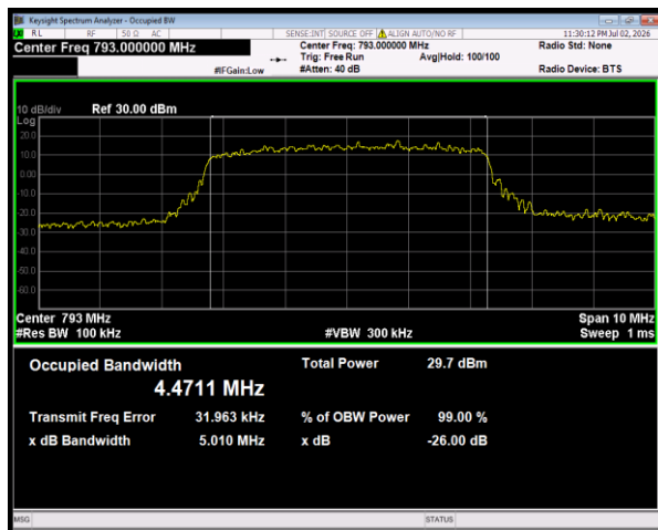
Band14 QPSK BW=5MHz Channel=23330 RB Size=25 Position=#0
