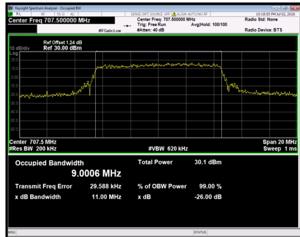
Band12 QPSK BW=10MHz Channel=23095 RB Size=50 Position=#0
