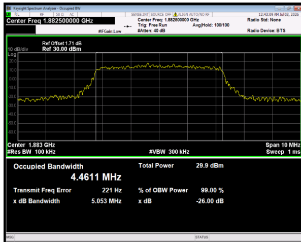
Band25 QPSK BW=5MHz Channel=26365 RB Size=25 Position=#0
