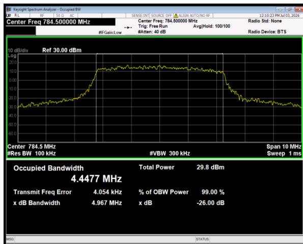
Band13 QPSK BW=5MHz Channel=23255 RB Size=25 Position=#0
