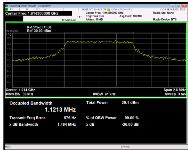
Band25 16QAM BW=1.4MHz Channel=26683 RB Size=6 Position=#0
