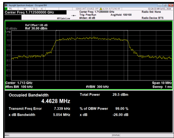
Band66 16QAM BW=5MHz Channel=131997 RB Size=25 Position=#0
