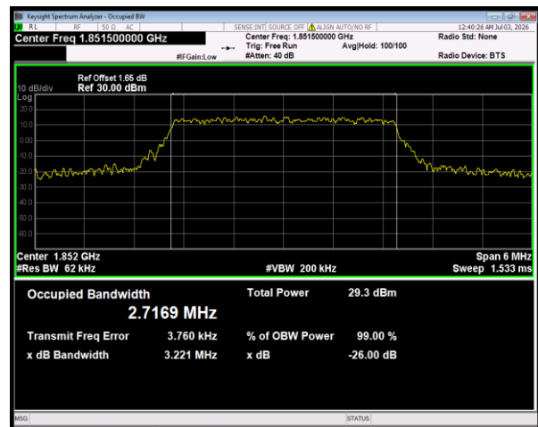
Band25 16QAM BW=3MHz Channel=26055 RB Size=15 Position=#0
