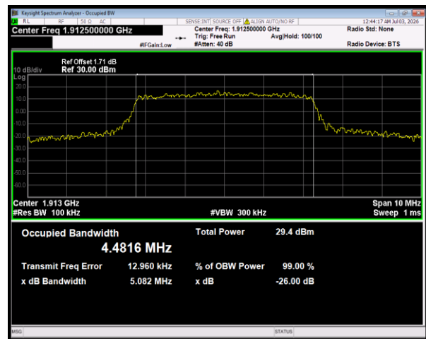
Band25 16QAM BW=5MHz Channel=26665 RB Size=25 Position=#0
