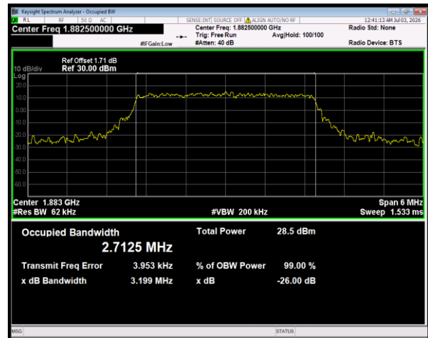
Band25 16QAM BW=3MHz Channel=26365 RB Size=15 Position=#0
