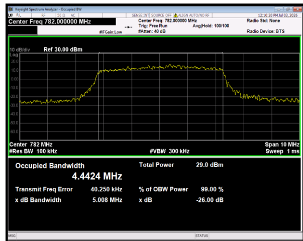
Band13 16QAM BW=5MHz Channel=23230 RB Size=25 Position=#0
