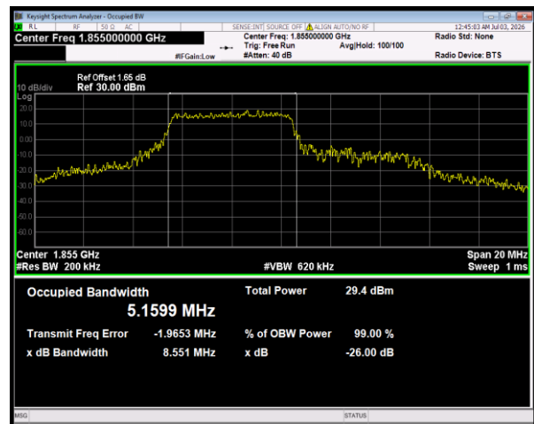
Band25 16QAM BW=10MHz Channel=26090 RB Size=27 Position=#0
