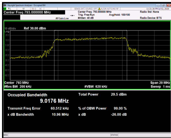
Band14 QPSK BW=10MHz Channel=23330 RB Size=50 Position=#0
