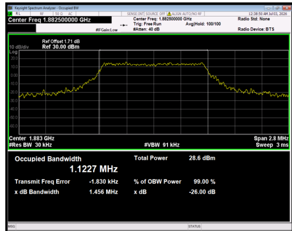
Band25 16QAM BW=1.4MHz Channel=26365 RB Size=6 Position=#0
