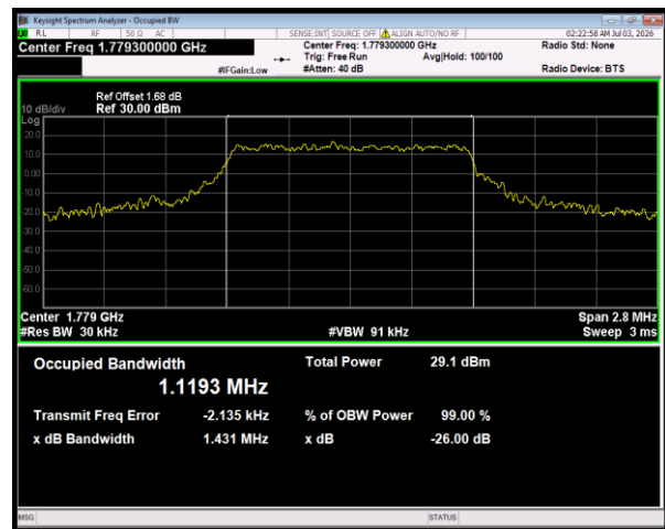
Band66 16QAM BW=1.4MHz Channel=132665 RB Size=6 Position=#0
