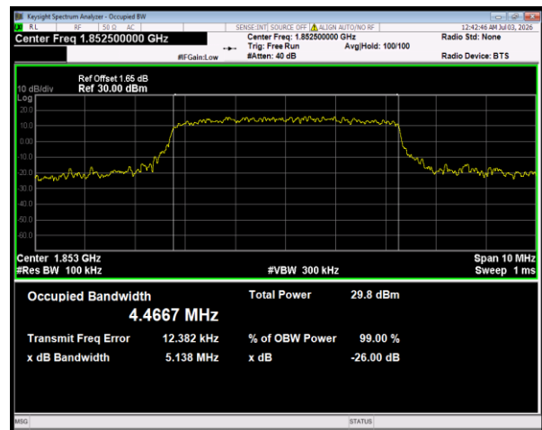
Band25 16QAM BW=5MHz Channel=26065 RB Size=25 Position=#0
