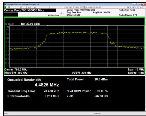
Band14 16QAM BW=5MHz Channel=23305 RB Size=25 Position=#0
