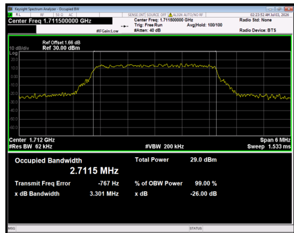
Band66 16QAM BW=3MHz Channel=131987 RB Size=15 Position=#0
