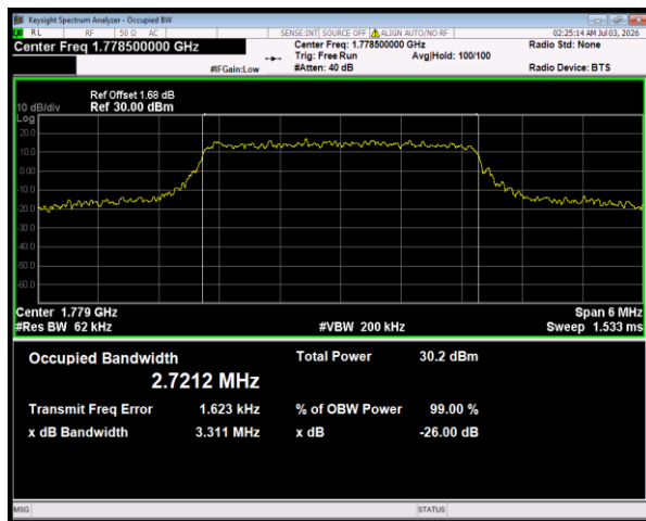
Band66 QPSK BW=3MHz Channel=132657 RB Size=15 Position=#0
