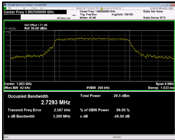
Band25 QPSK BW=3MHz Channel=26365 RB Size=15 Position=#0
