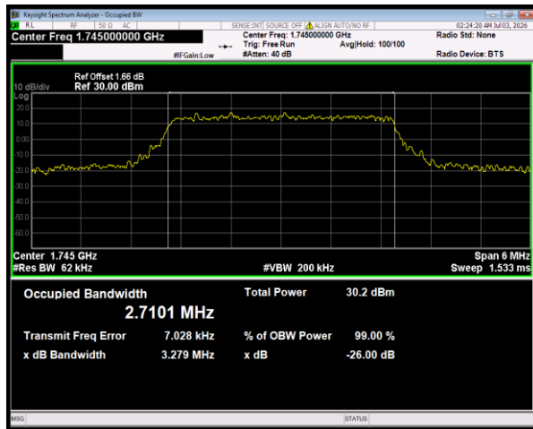
Band66 QPSK BW=3MHz Channel=132322 RB Size=15 Position=#0
