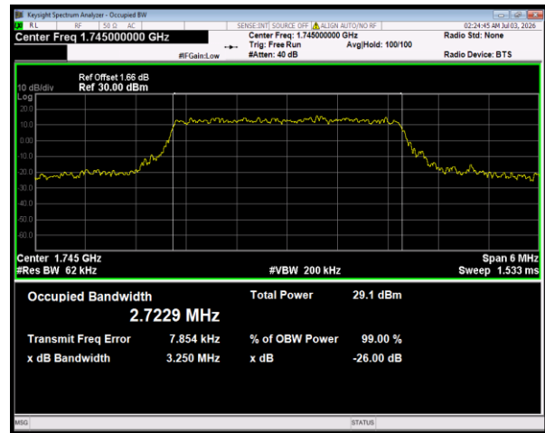
Band66 16QAM BW=3MHz Channel=132322 RB Size=15 Position=#0
