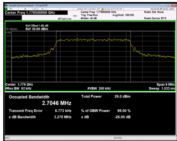
Band66 16QAM BW=3MHz Channel=132657 RB Size=15 Position=#0
