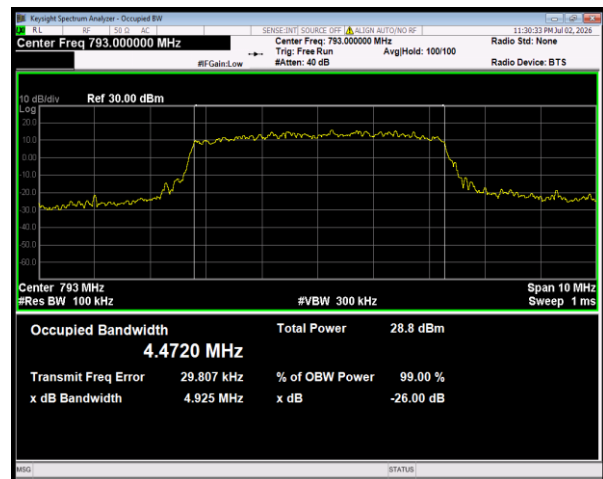
Band14 16QAM BW=5MHz Channel=23330 RB Size=25 Position=#0
