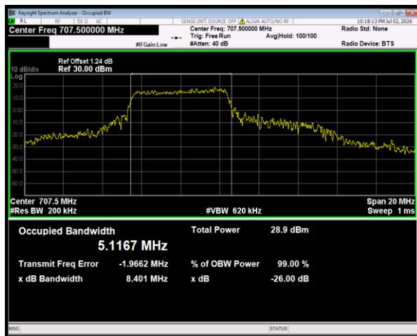
Band12 16QAM BW=10MHz Channel=23095 RB Size=27 Position=#0
