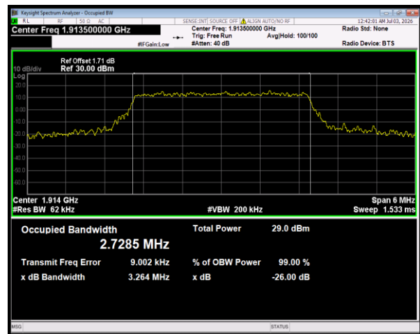
Band25 16QAM BW=3MHz Channel=26675 RB Size=15 Position=#0
