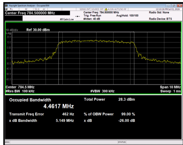
Band13 16QAM BW=5MHz Channel=23255 RB Size=25 Position=#0
