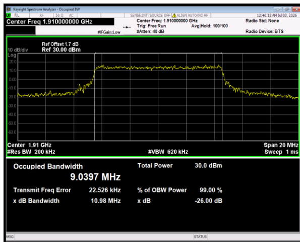
Band25 QPSK BW=10MHz Channel=26640 RB Size=50 Position=#0
