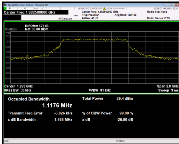
Band25 QPSK BW=1.4MHz Channel=26365 RB Size=6 Position=#0
