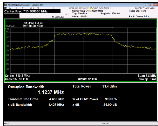
Band12 16QAM BW=1.4MHz Channel=23173 RB Size=6 Position=#0
