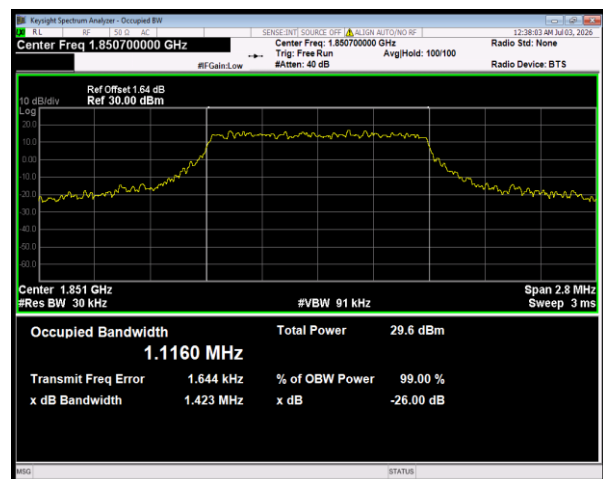
Band25 16QAM BW=1.4MHz Channel=26047 RB Size=6 Position=#0
