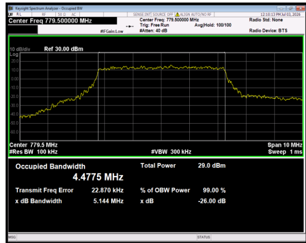
Band13 16QAM BW=5MHz Channel=23205 RB Size=25 Position=#0
