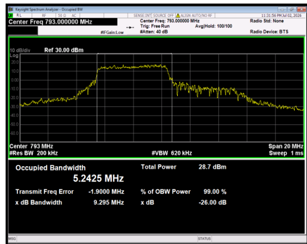
Band14 16QAM BW=10MHz Channel=23330 RB Size=27 Position=#0
