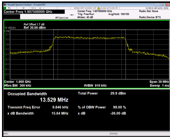
Band25 QPSK BW=15MHz Channel=26615 RB Size=75 Position=#0
