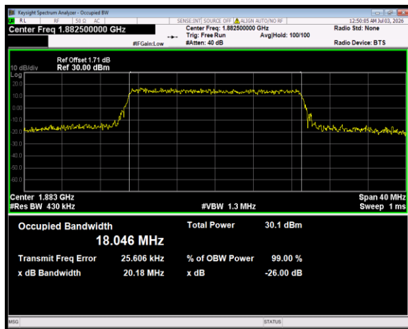
Band25 QPSK BW=20MHz Channel=26365 RB Size=100 Position=#0
