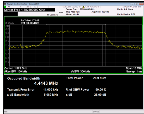
Band25 16QAM BW=5MHz Channel=26365 RB Size=25 Position=#0
