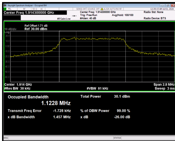
Band25 QPSK BW=1.4MHz Channel=26683 RB Size=6 Position=#0
