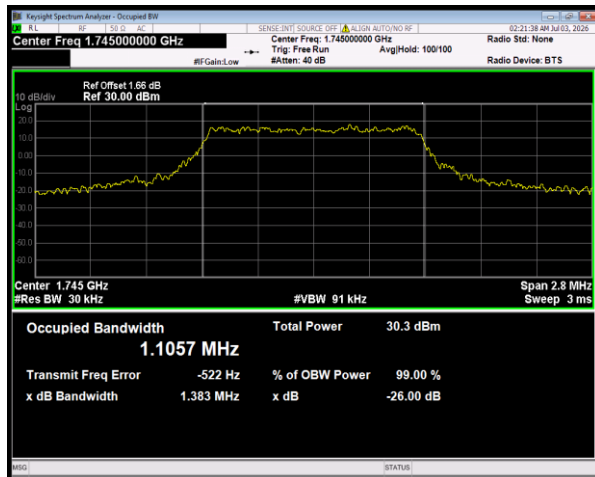
Band66 QPSK BW=1.4MHz Channel=132322 RB Size=6 Position=#0
