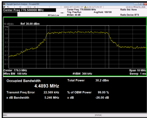
Band13 QPSK BW=5MHz Channel=23205 RB Size=25 Position=#0
