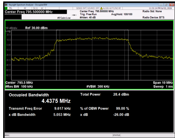
Band14 16QAM BW=5MHz Channel=23355 RB Size=25 Position=#0
