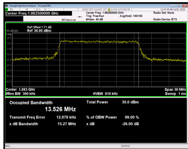
Band25 QPSK BW=15MHz Channel=26365 RB Size=75 Position=#0
