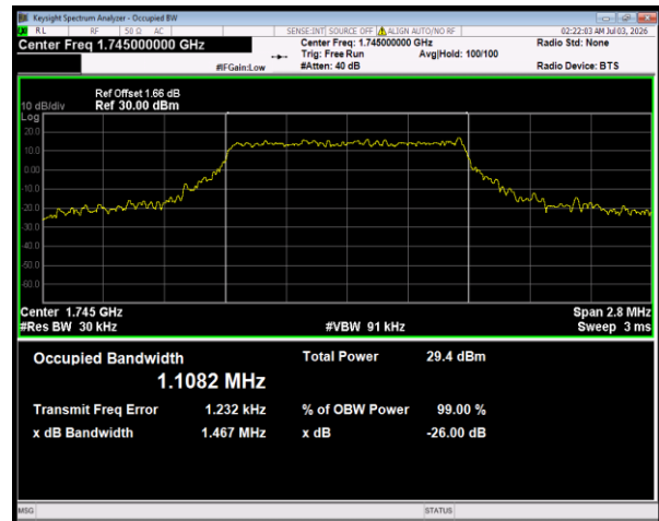
Band66 16QAM BW=1.4MHz Channel=132322 RB Size=6 Position=#0
