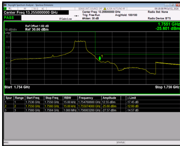
Band4 16QAM BW=1.4MHz HighChannel=20393 RB Size=1 Position=#Max
