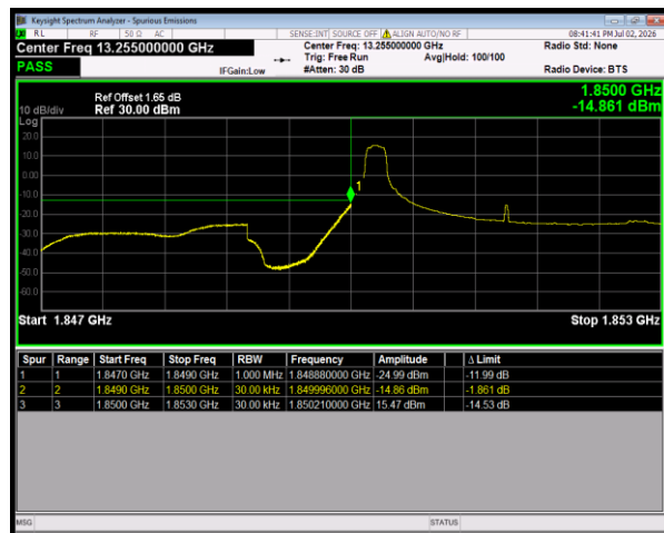
Band2 16QAM BW=3MHz LowChannel=18615 RB Size=1 Position=#0
