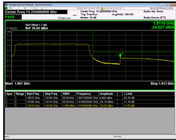
Band2 QPSK BW=3MHz HighChannel=19185 RB Size=15 Position=#0
