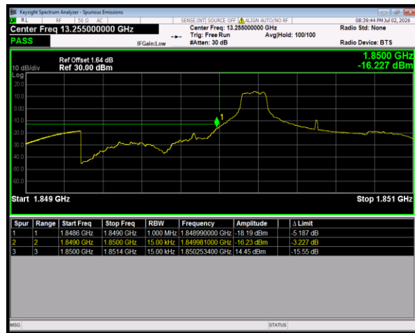
Band2 QPSK BW=1.4MHz LowChannel=18607 RB Size=1 Position=#0
