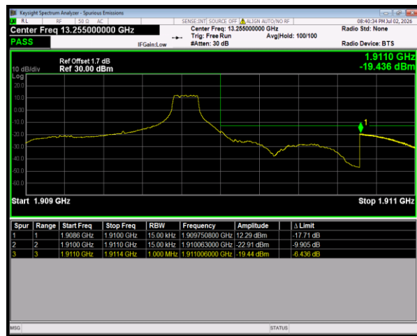
Band2 16QAM BW=1.4MHz HighChannel=19193 RB Size=1 Position=#Max
