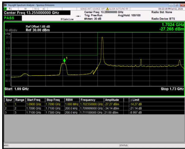
Band4 16QAM BW=20MHz LowChannel=20050 RB Size=1 Position=#0
