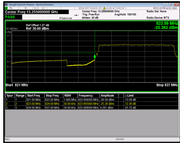
Band5 QPSK BW=3MHz LowChannel=20415 RB Size=15 Position=#0
