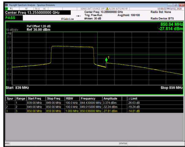
Band5 16QAM BW=10MHz HighChannel=20600 RB Size=27 Position=#Max
