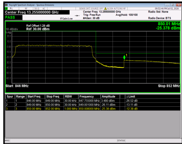
Band5 QPSK BW=3MHz HighChannel=20635 RB Size=15 Position=#0
