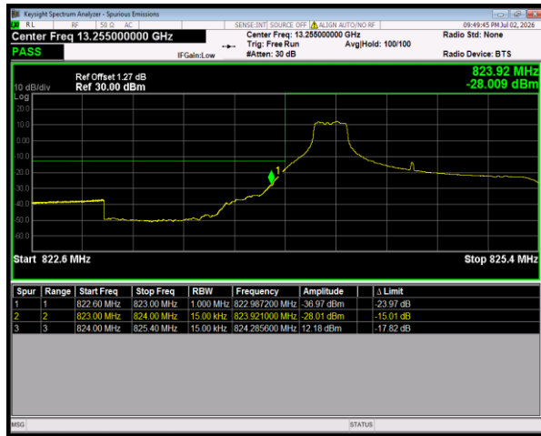
Band5 16QAM BW=1.4MHz LowChannel=20407 RB Size=1 Position=#0
