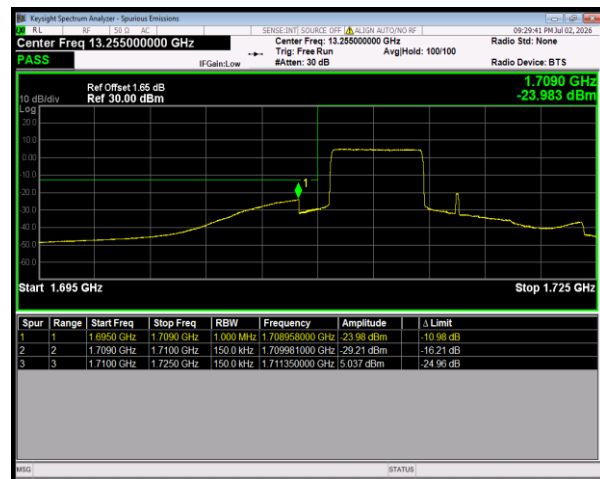
Band4 16QAM BW=15MHz LowChannel=20025 RB Size=27 Position=#0
