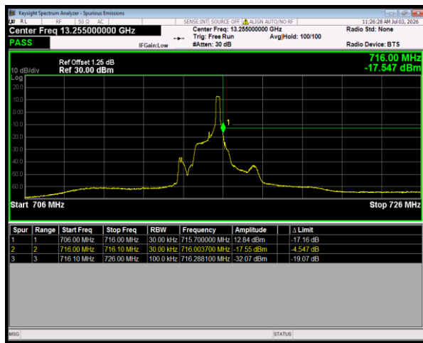
Band12 16QAM BW=1.4MHz HighChannel=23173 RB Size=1 Position=#Max
