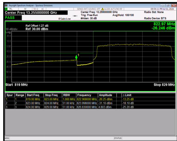
Band5 QPSK BW=5MHz LowChannel=20425 RB Size=25 Position=#0
