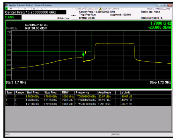
Band4 16QAM BW=10MHz LowChannel=20000 RB Size=27 Position=#0
