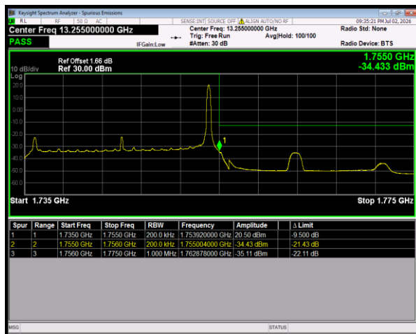
Band4 16QAM BW=20MHz HighChannel=20300 RB Size=1 Position=#Max
