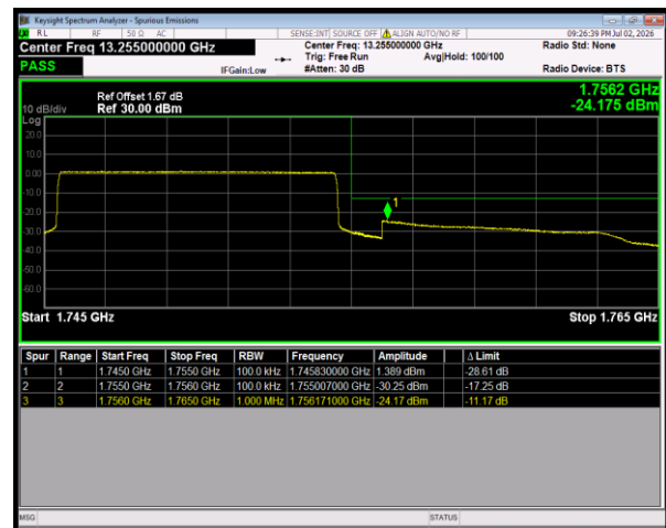
Band4 QPSK BW=10MHz HighChannel=20350 RB Size=50 Position=#0
