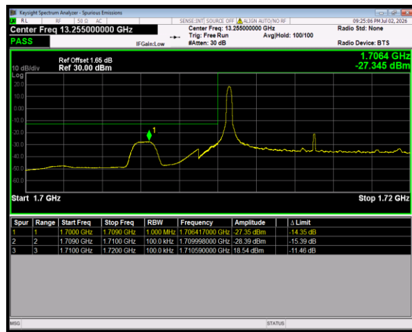
Band4 16QAM BW=10MHz LowChannel=20000 RB Size=1 Position=#0
