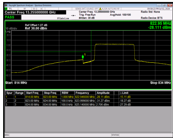
Band5 16QAM BW=10MHz LowChannel=20450 RB Size=27 Position=#0
