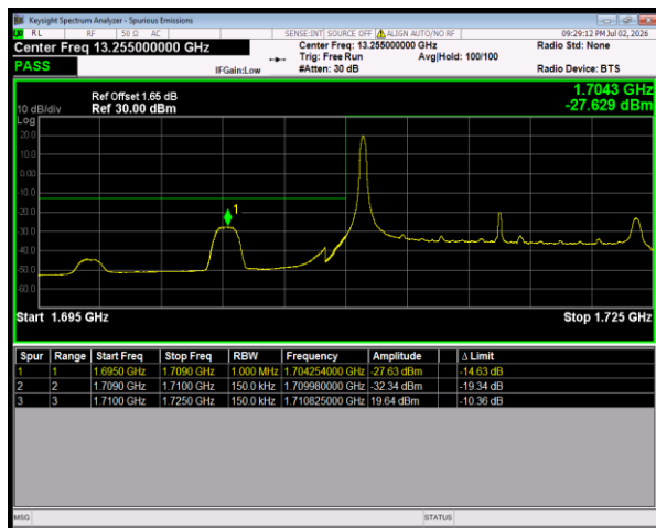
Band4 16QAM BW=15MHz LowChannel=20025 RB Size=1 Position=#0
