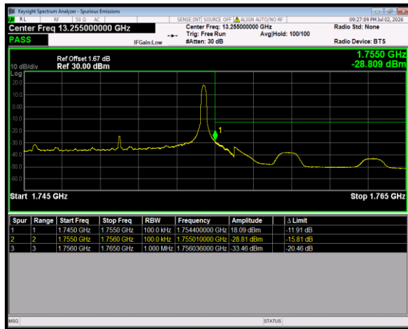
Band4 16QAM BW=10MHz HighChannel=20350 RB Size=1 Position=#Max
