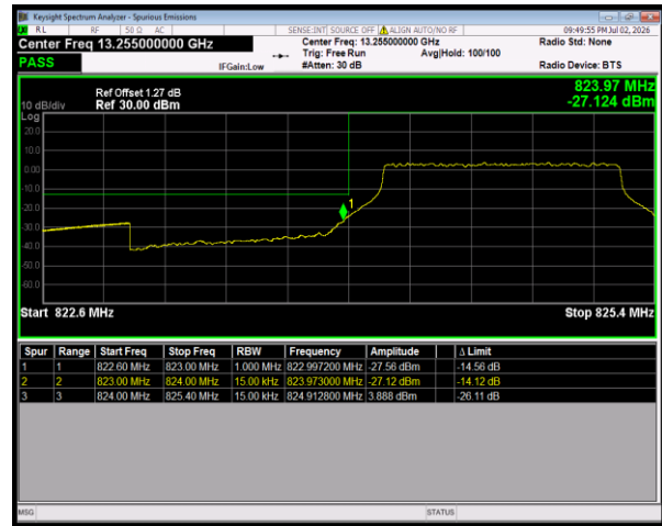
Band5 16QAM BW=1.4MHz LowChannel=20407 RB Size=6 Position=#0
