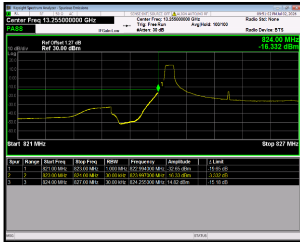
Band5 QPSK BW=3MHz LowChannel=20415 RB Size=1 Position=#0
