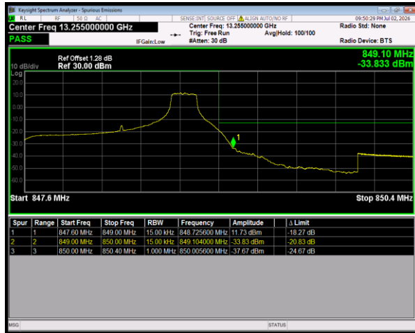
Band5 16QAM BW=1.4MHz HighChannel=20643 RB Size=1 Position=#Max
