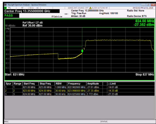
Band5 16QAM BW=3MHz LowChannel=20415 RB Size=15 Position=#0
