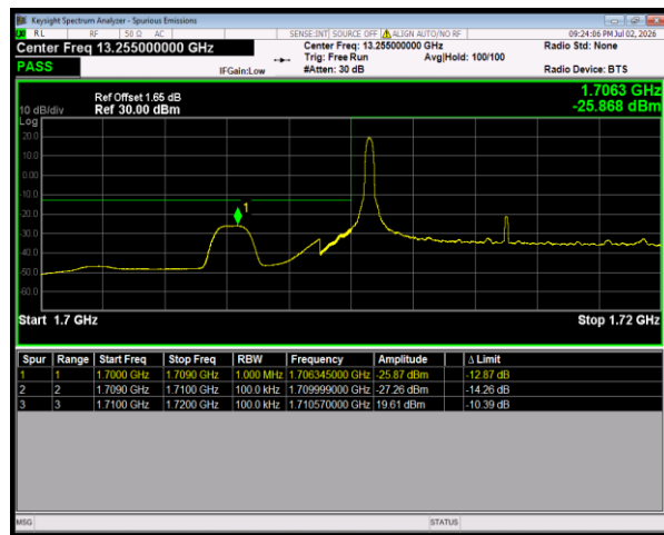
Band4 QPSK BW=10MHz LowChannel=20000 RB Size=1 Position=#0
