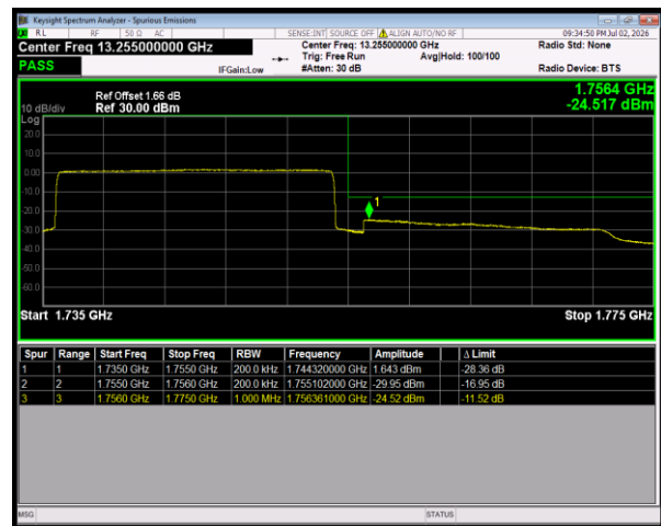
Band4 QPSK BW=20MHz HighChannel=20300 RB Size=100 Position=#0
