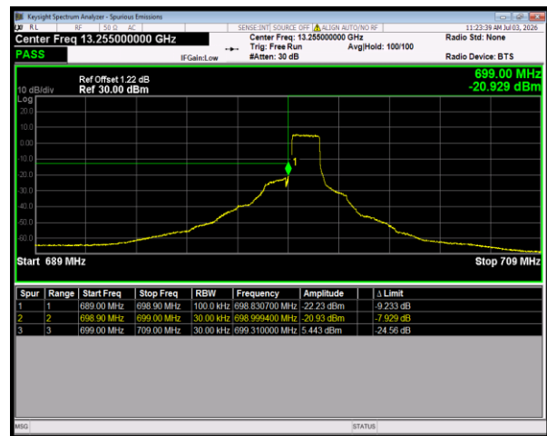
Band12 QPSK BW=1.4MHz LowChannel=23017 RB Size=6 Position=#0
