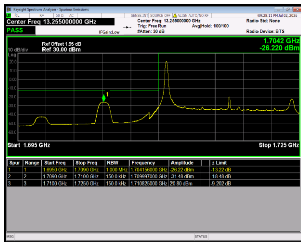
Band4 QPSK BW=15MHz LowChannel=20025 RB Size=1 Position=#0
