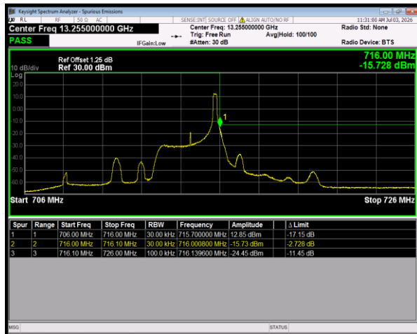
Band12 16QAM BW=3MHz HighChannel=23165 RB Size=1 Position=#Max
