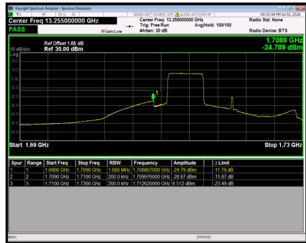
Band4 16QAM BW=20MHz LowChannel=20050 RB Size=27 Position=#0
