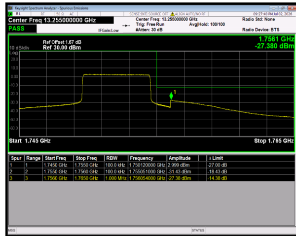
Band4 16QAM BW=10MHz HighChannel=20350 RB Size=27 Position=#Max
