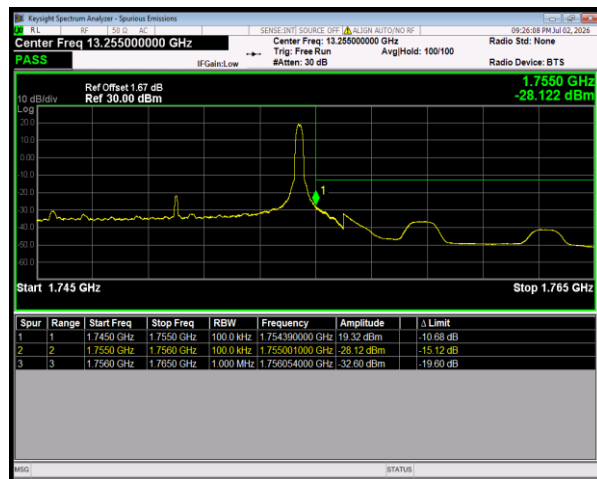
Band4 QPSK BW=10MHz HighChannel=20350 RB Size=1 Position=#Max
