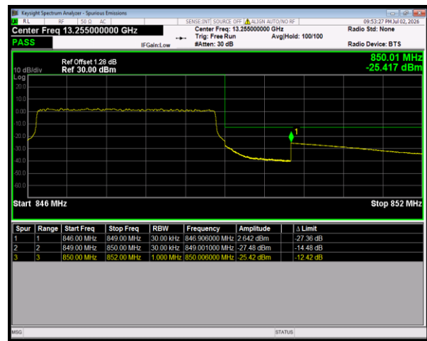
Band5 16QAM BW=3MHz HighChannel=20635 RB Size=15 Position=#0
