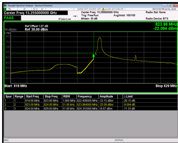
Band5 QPSK BW=5MHz LowChannel=20425 RB Size=1 Position=#0
