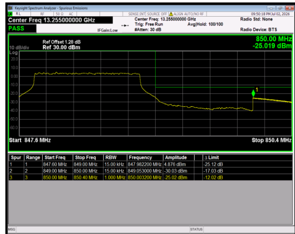
Band5 QPSK BW=1.4MHz HighChannel=20643 RB Size=6 Position=#0
