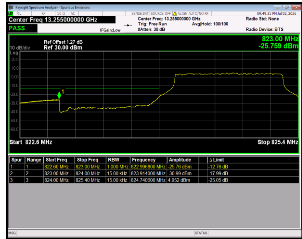
Band5 QPSK BW=1.4MHz LowChannel=20407 RB Size=6 Position=#0
