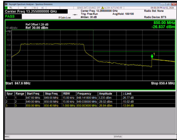
Band5 16QAM BW=1.4MHz HighChannel=20643 RB Size=6 Position=#0
