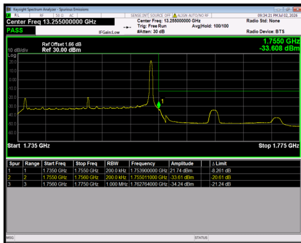
Band4 QPSK BW=20MHz HighChannel=20300 RB Size=1 Position=#Max
