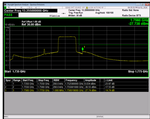
Band4 16QAM BW=20MHz HighChannel=20300 RB Size=27 Position=#Max
