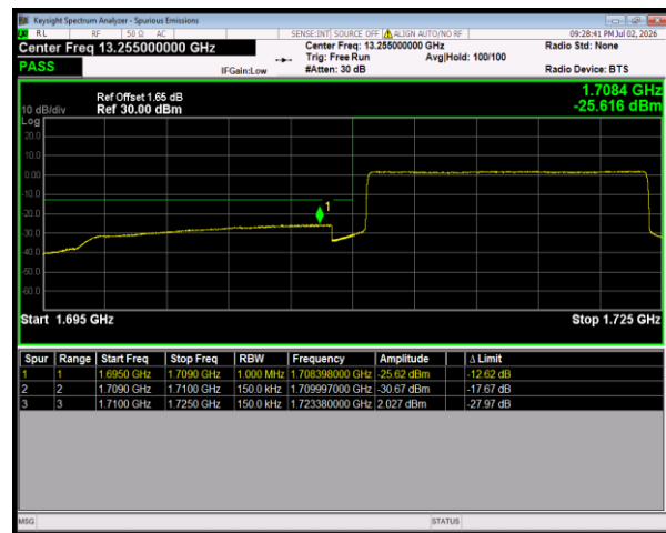
Band4 QPSK BW=15MHz LowChannel=20025 RB Size=75 Position=#0
