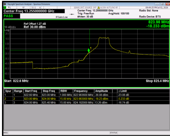
Band5 QPSK BW=1.4MHz LowChannel=20407 RB Size=1 Position=#0
