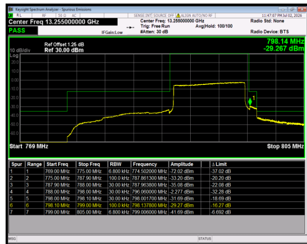
Band14 QPSK BW=10MHz HighChannel=23330 RB Size=50 Position=#0
