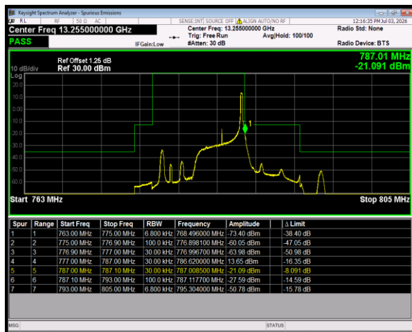
Band13 16QAM BW=5MHz HighChannel=23255 RB Size=1 Position=#Max
