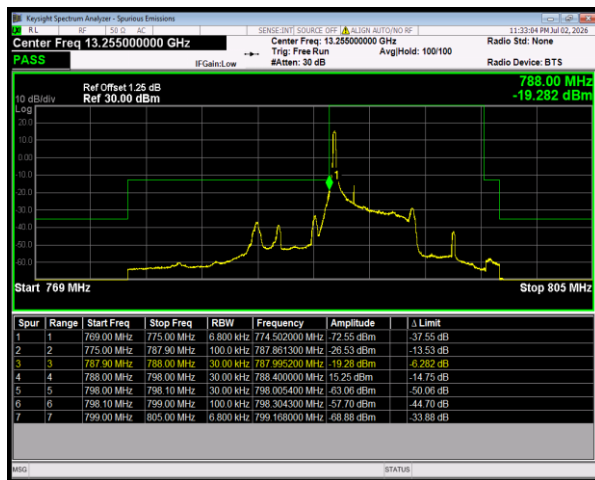
Band14 QPSK BW=5MHz LowChannel=23305 RB Size=1 Position=#0
