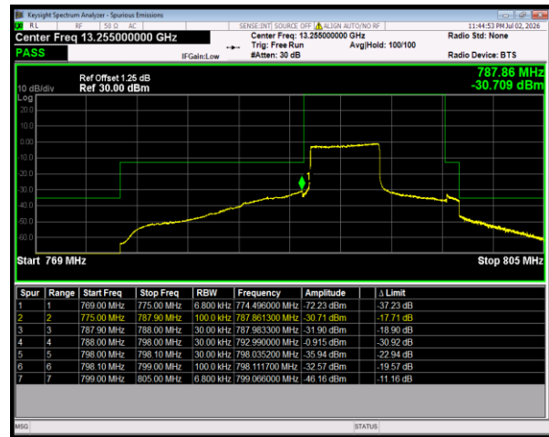
Band14 16QAM BW=10MHz LowChannel=23330 RB Size=27 Position=#0
