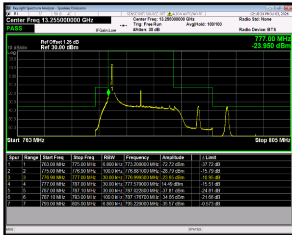
Band13 QPSK BW=10MHz LowChannel=23230 RB Size=1 Position=#0
