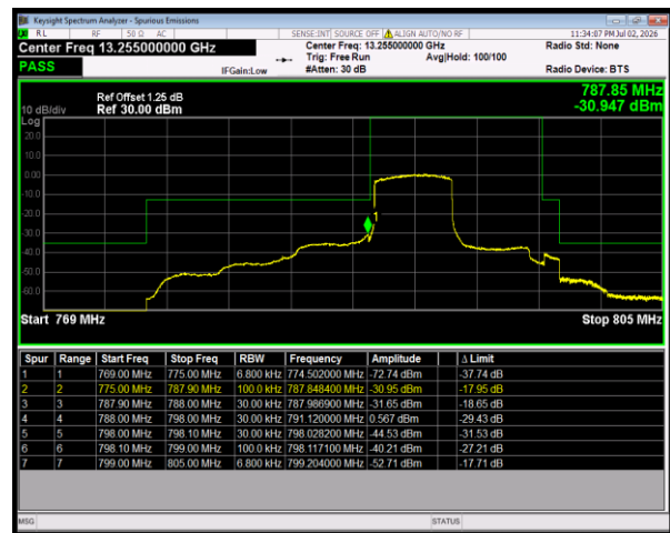
Band14 QPSK BW=5MHz LowChannel=23305 RB Size=25 Position=#0
