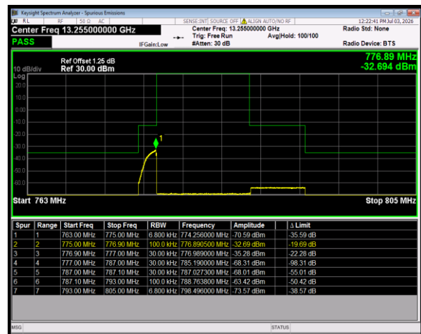
Band13 QPSK BW=10MHz HighChannel=23230 RB Size=50 Position=#0
