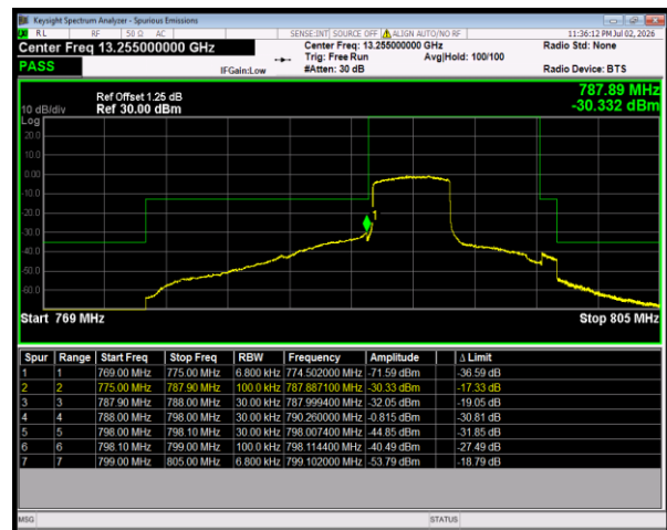
Band14 16QAM BW=5MHz LowChannel=23305 RB Size=25 Position=#0
