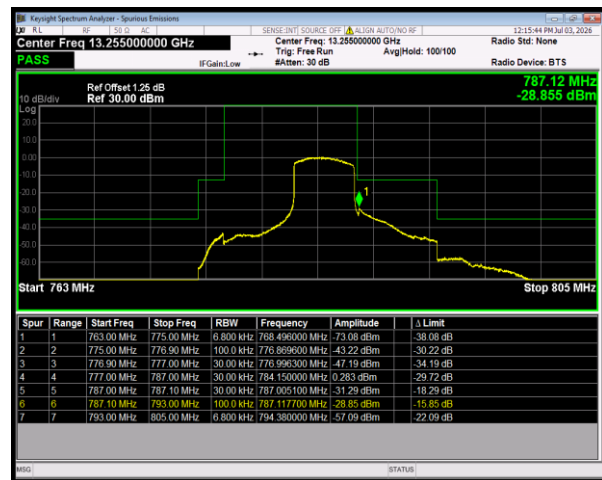
Band13 QPSK BW=5MHz HighChannel=23255 RB Size=25 Position=#0
