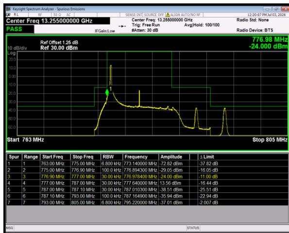
Band13 16QAM BW=10MHz LowChannel=23230 RB Size=1 Position=#0
