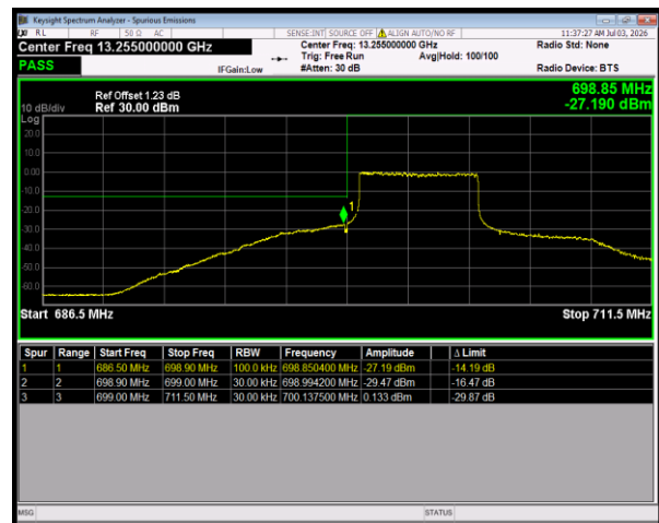
Band12 16QAM BW=10MHz LowChannel=23060 RB Size=27 Position=#0
