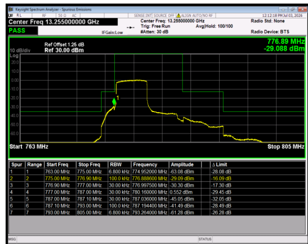
Band13 QPSK BW=5MHz LowChannel=23205 RB Size=25 Position=#0
