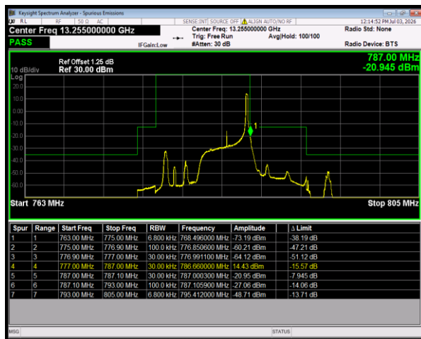
Band13 QPSK BW=5MHz HighChannel=23255 RB Size=1 Position=#Max
