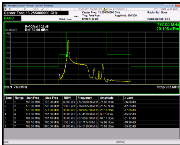
Band13 QPSK BW=5MHz LowChannel=23205 RB Size=1 Position=#0
