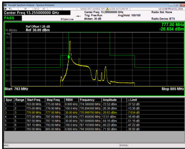
Band13 16QAM BW=5MHz LowChannel=23205 RB Size=1 Position=#0
