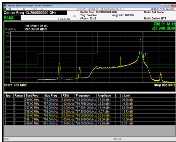
Band14 QPSK BW=10MHz HighChannel=23330 RB Size=1 Position=#Max
