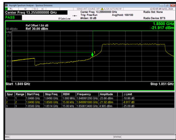
Band25 16QAM BW=1.4MHz LowChannel=26047 RB Size=6 Position=#0
