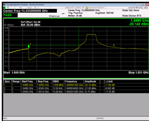
Band25 16QAM BW=1.4MHz LowChannel=26047 RB Size=1 Position=#0
