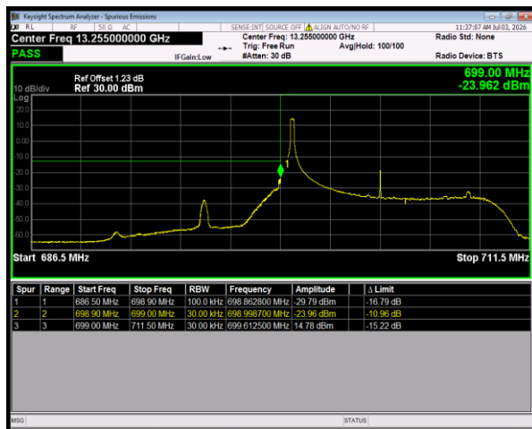
Band12 16QAM BW=10MHz LowChannel=23060 RB Size=1 Position=#0
