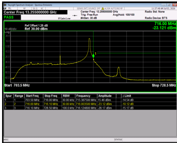
Band12 QPSK BW=10MHz HighChannel=23130 RB Size=1 Position=#Max
