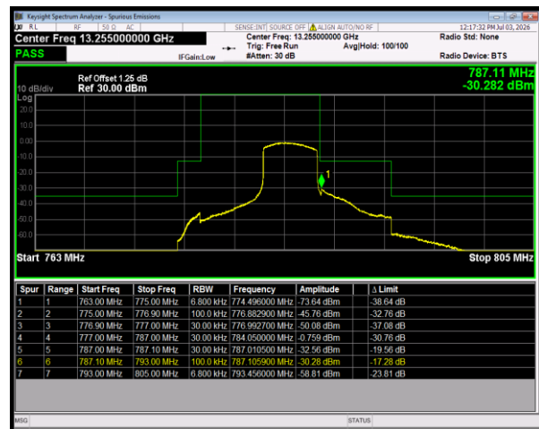
Band13 16QAM BW=5MHz HighChannel=23255 RB Size=25 Position=#0
