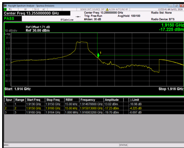
Band25 QPSK BW=1.4MHz HighChannel=26683 RB Size=1 Position=#Max
