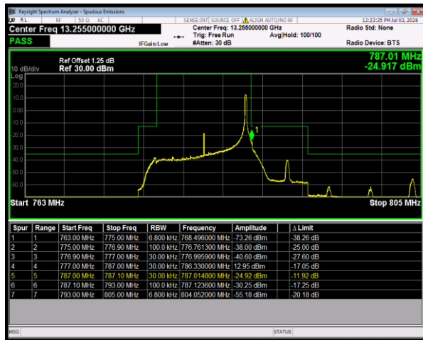
Band13 16QAM BW=10MHz HighChannel=23230 RB Size=1 Position=#Max
