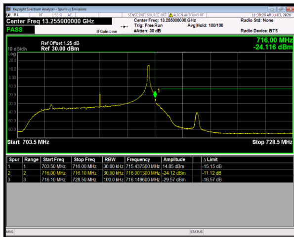
Band12 16QAM BW=10MHz HighChannel=23130 RB Size=1 Position=#Max
