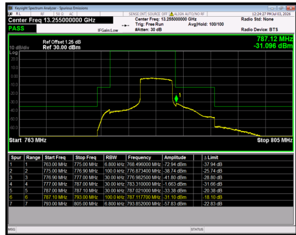
Band13 16QAM BW=10MHz HighChannel=23230 RB Size=27 Position=#Max
