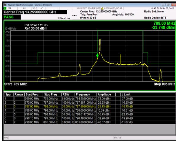
Band14 16QAM BW=10MHz LowChannel=23330 RB Size=1 Position=#0
