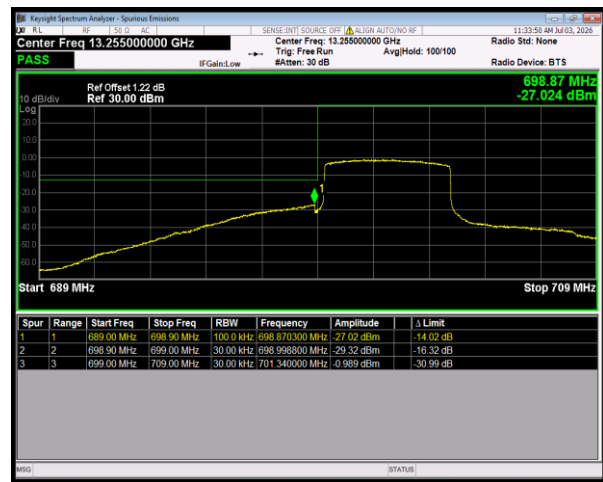
Band12 16QAM BW=5MHz LowChannel=23035 RB Size=25 Position=#0
