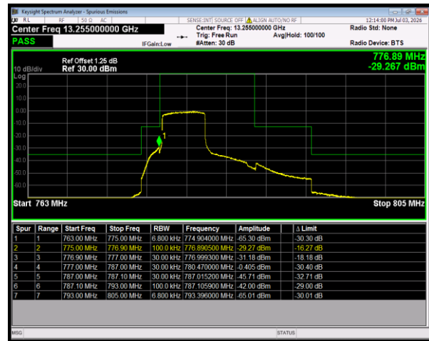
Band13 16QAM BW=5MHz LowChannel=23205 RB Size=25 Position=#0
