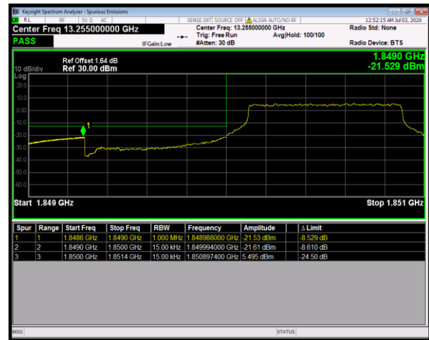
Band25 QPSK BW=1.4MHz LowChannel=26047 RB Size=6 Position=#0
