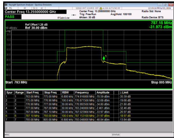
Band13 QPSK BW=10MHz LowChannel=23230 RB Size=50 Position=#0
