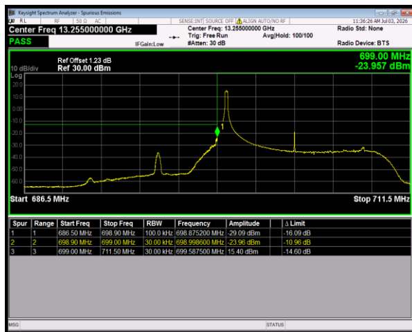
Band12 QPSK BW=10MHz LowChannel=23060 RB Size=1 Position=#0
