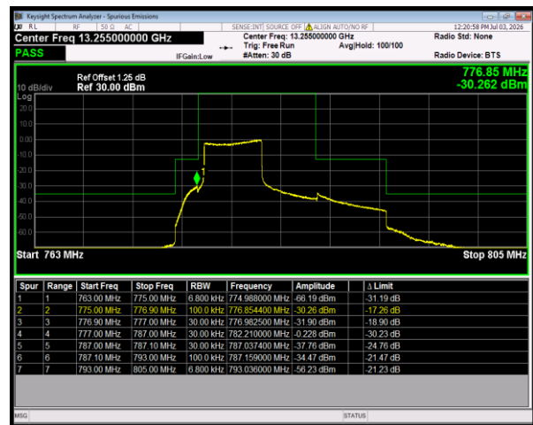
Band13 16QAM BW=10MHz LowChannel=23230 RB Size=27 Position=#0
