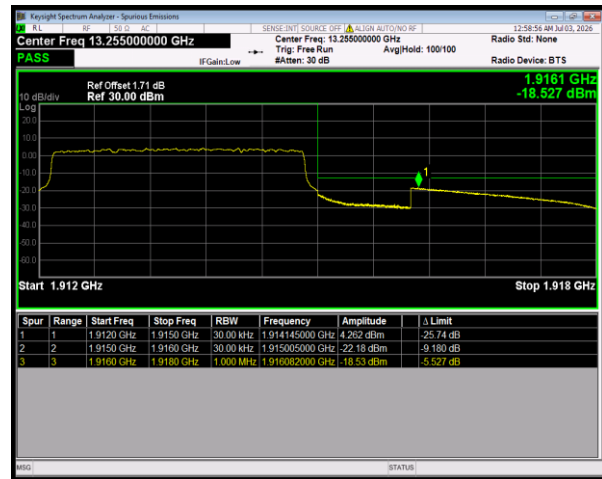
Band25 QPSK BW=3MHz HighChannel=26675 RB Size=15
