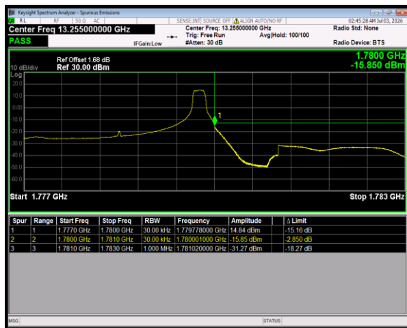
Band66 16QAM BW=3MHz HighChannel=132657 RB Size=1 Position=#Max
