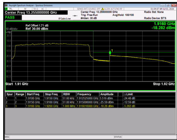
Band25 QPSK BW=5MHz HighChannel=26665 RB Size=25 Position=#0
