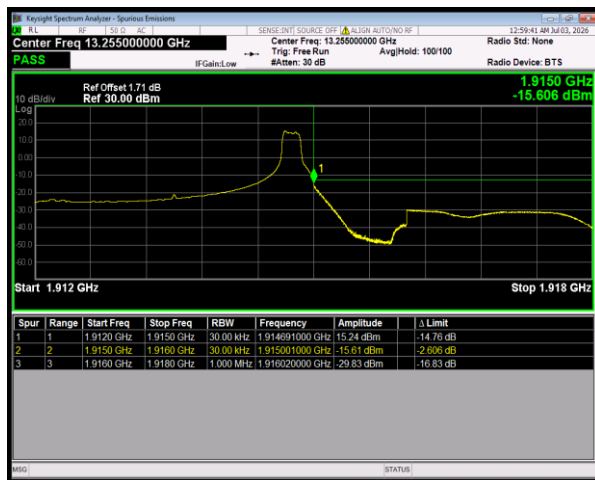
Band25 16QAM BW=3MHz HighChannel=26675 RB Size=1
