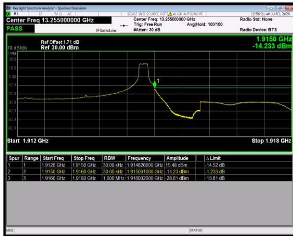
Band25 QPSK BW=3MHz HighChannel=26675 RB Size=1
