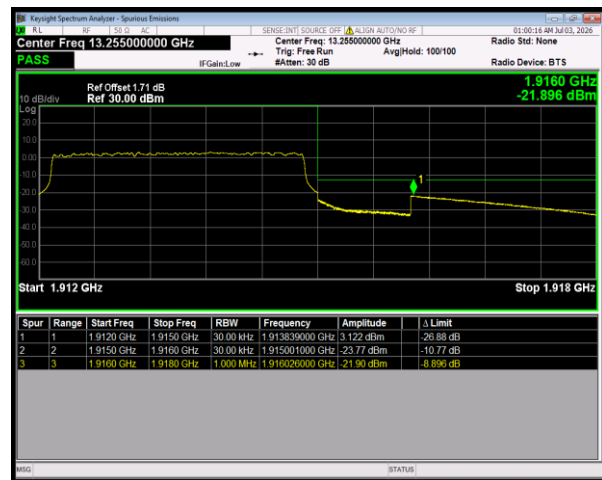
Band25 16QAM BW=3MHz HighChannel=26675 RB Size=15
