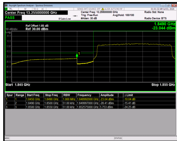
Band25 QPSK BW=5MHz LowChannel=26065 RB Size=25
