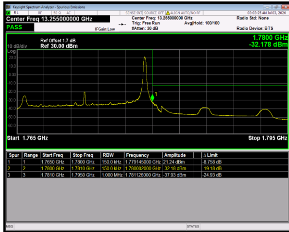
Band66 QPSK BW=15MHz HighChannel=132597 RB Size=1 Position=#Max
