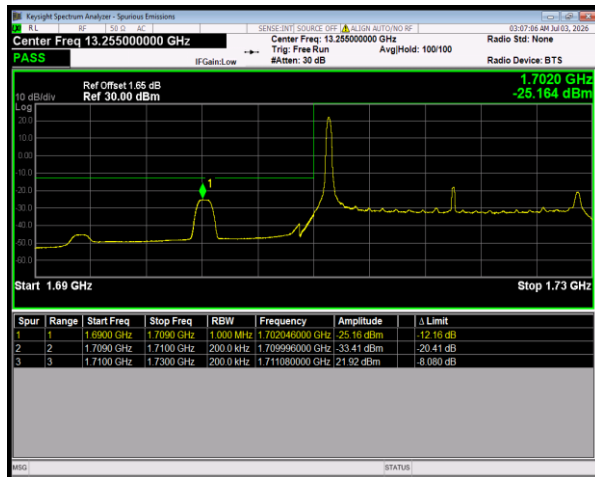
Band66 QPSK BW=20MHz LowChannel=132072 RB Size=1 Position=#0
