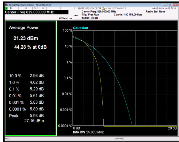
Band5 16QAM BW=10MHz Channel=20450 RB Size=27 Position=#0
