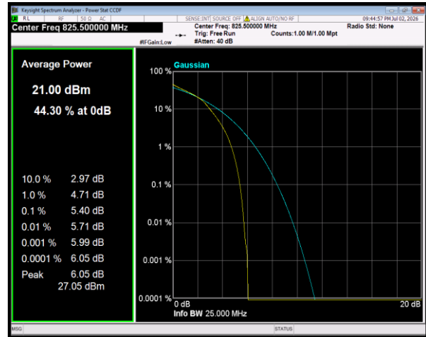
Band5 16QAM BW=3MHz Channel=20415 RB Size=15 Position=#0
