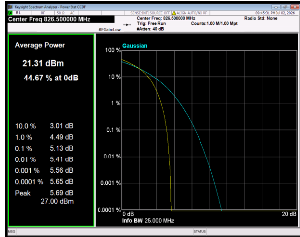
Band5 16QAM BW=5MHz Channel=20425 RB Size=25 Position=#0
