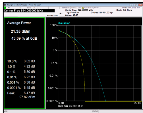
Band5 16QAM BW=10MHz Channel=20600 RB Size=27 Position=#0
