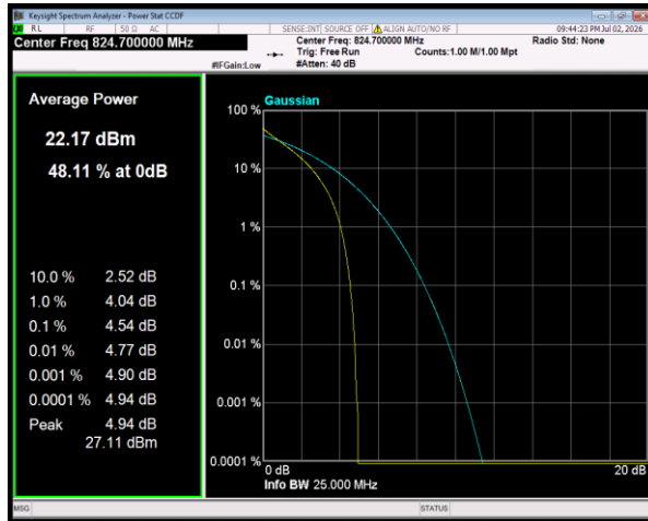
Band5 QPSK BW=1.4MHz Channel=20407 RB Size=6 Position=#0
