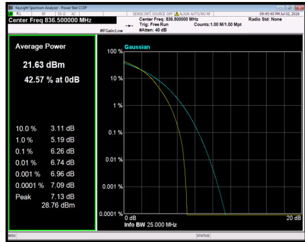
Band5 16QAM BW=5MHz Channel=20525 RB Size=25 Position=#0
