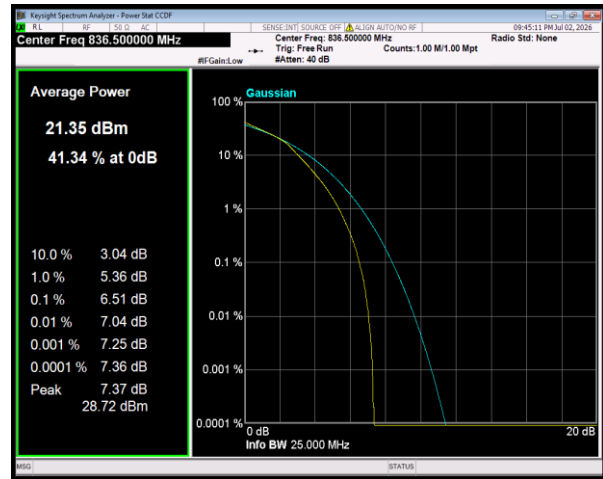
Band5 16QAM BW=3MHz Channel=20525 RB Size=15 Position=#0
