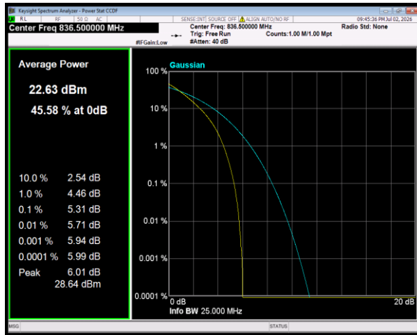
Band5 QPSK BW=5MHz Channel=20525 RB Size=25 Position=#0
