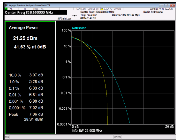
Band5 16QAM BW=10MHz Channel=20525 RB Size=27 Position=#0
