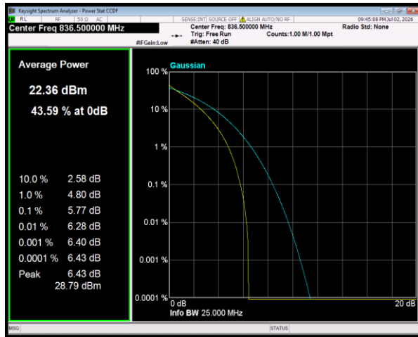
Band5 QPSK BW=3MHz Channel=20525 RB Size=15 Position=#0
