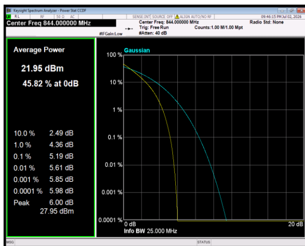
Band5 QPSK BW=10MHz Channel=20600 RB Size=50 Position=#0
