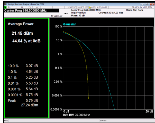
Band5 16QAM BW=5MHz Channel=20625 RB Size=25 Position=#0
