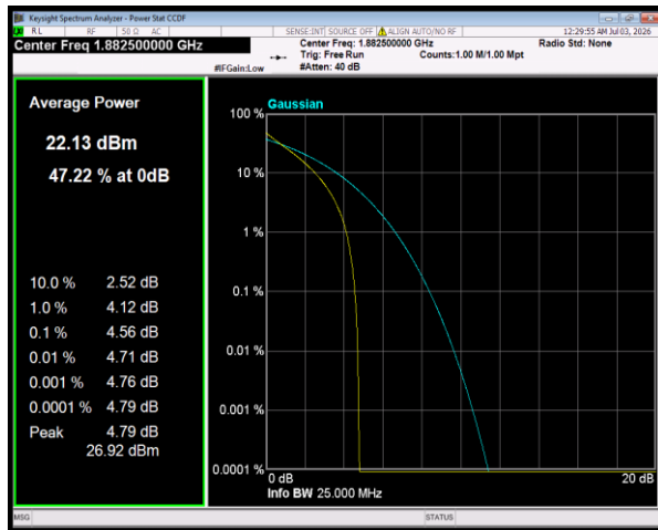
Band25 QPSK BW=3MHz Channel=26365 RB Size=15 Position=#0
