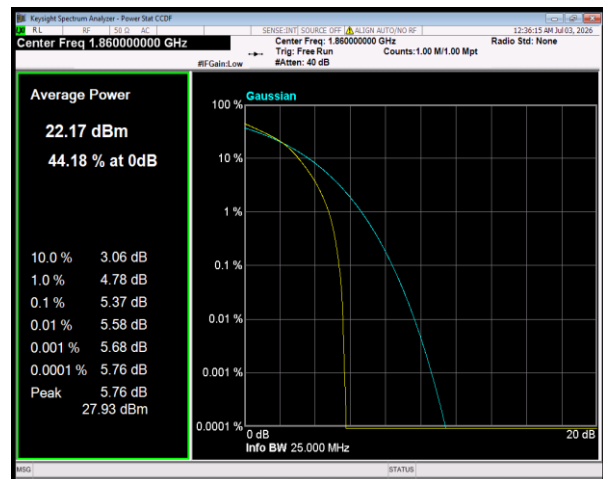
Band25 16QAM BW=20MHz Channel=26140 RB Size=27 Position=#0
