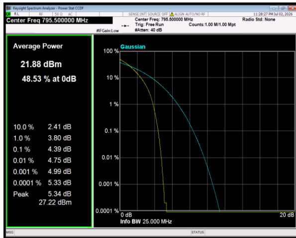
Band14 QPSK BW=5MHz Channel=23355 RB Size=25 Position=#0
