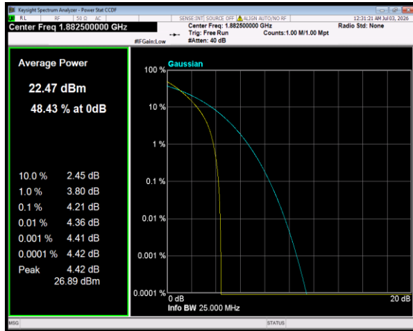
Band25 QPSK BW=5MHz Channel=26365 RB Size=25 Position=#0
