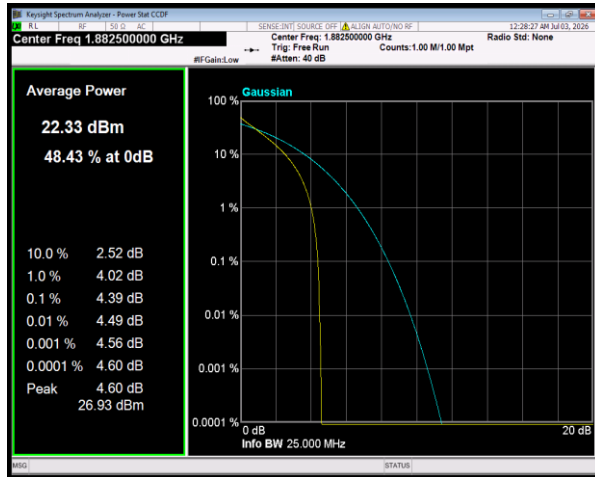
Band25 QPSK BW=1.4MHz Channel=26365 RB Size=6 Position=#0
