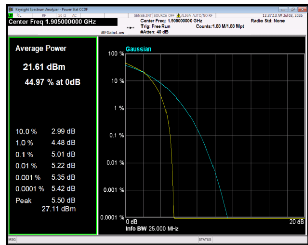
Band25 16QAM BW=20MHz Channel=26590 RB Size=27 Position=#0
