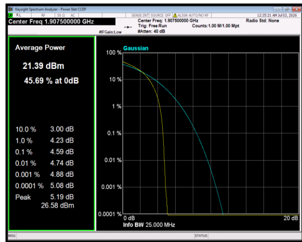
Band25 16QAM BW=15MHz Channel=26615 RB Size=27 Position=#0
