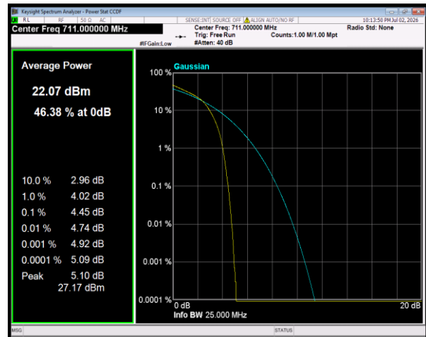
Band12 16QAM BW=10MHz Channel=23130 RB Size=27 Position=#0
