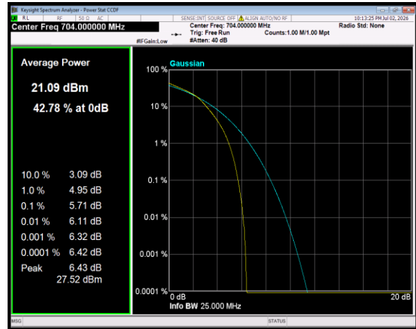
Band12 16QAM BW=10MHz Channel=23060 RB Size=27 Position=#0
