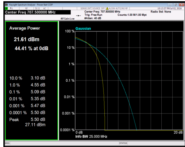
Band12 16QAM BW=10MHz Channel=23095 RB Size=27 Position=#0
