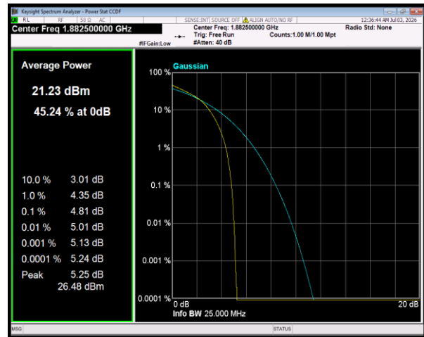
Band25 16QAM BW=20MHz Channel=26365 RB Size=27 Position=#0
