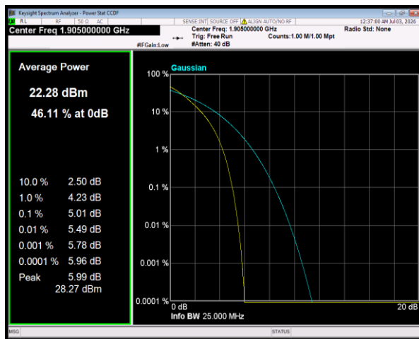
Band25 QPSK BW=20MHz Channel=26590 RB Size=100 Position=#0
