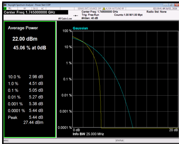
Band66 16QAM BW=20MHz Channel=132322 RB Size=27 Position=#0
