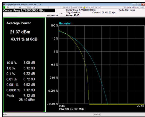
Band66 16QAM BW=20MHz Channel=132572 RB Size=27 Position=#0
