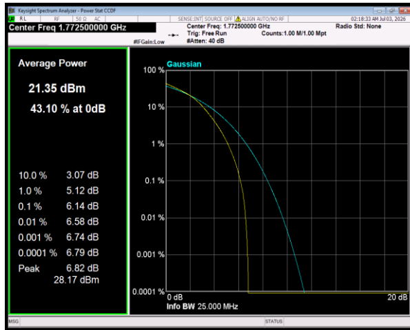
Band66 16QAM BW=15MHz Channel=132597 RB Size=27 Position=#0
