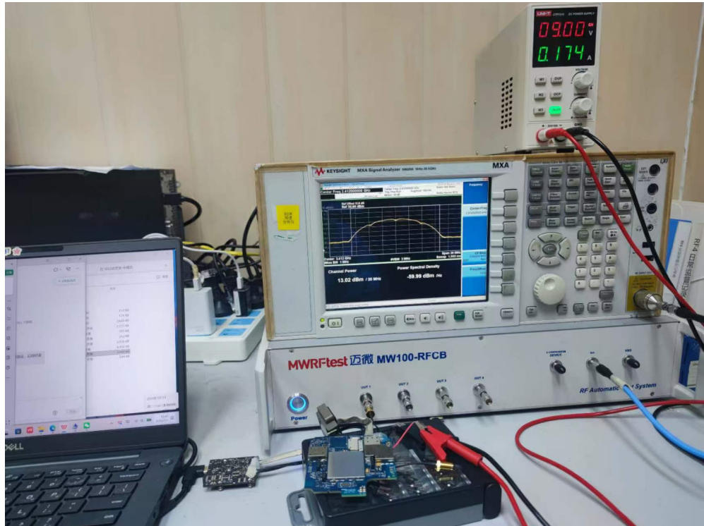
WLAN Test Setup
