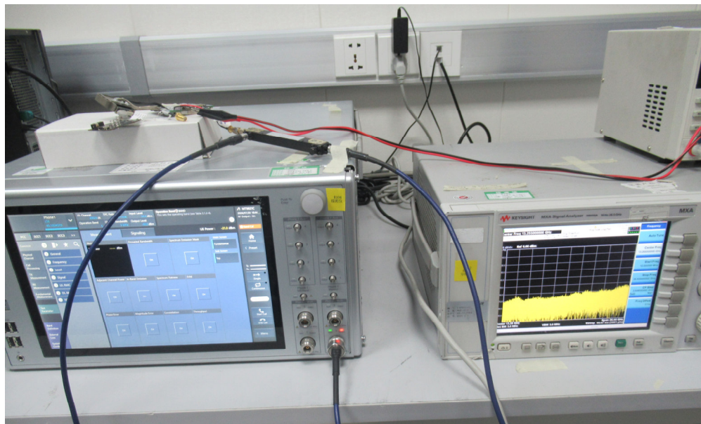
WWAN Test Setup
