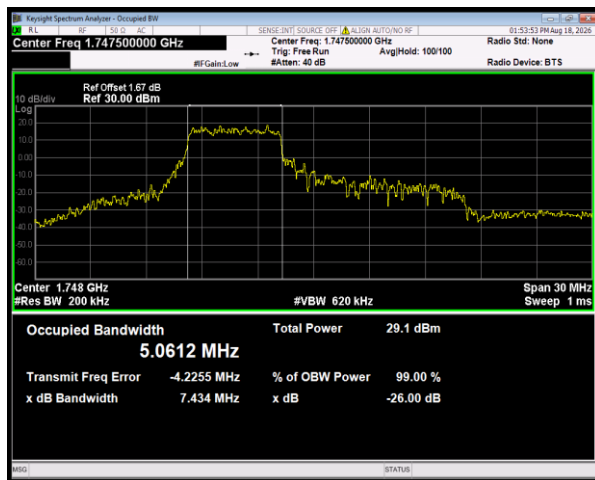
Band4 16QAM BW=15MHz Channel=20325 RB Size=27 Position=#0
