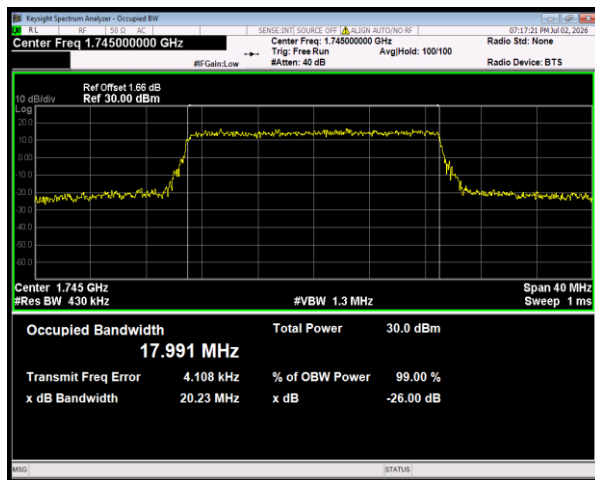
Band66 QPSK BW=20MHz Channel=132322 RB Size=100 Position=#0
