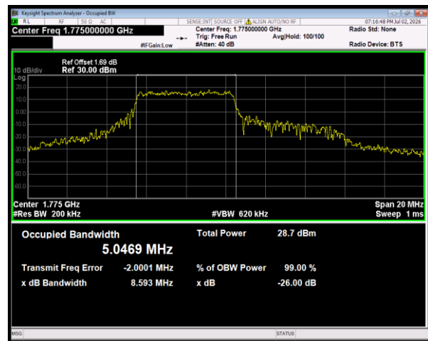
Band66 16QAM BW=10MHz Channel=132622 RB Size=27 Position=#0
