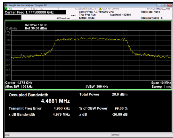
Band66 16QAM BW=5MHz Channel=132647 RB Size=25 Position=#0
