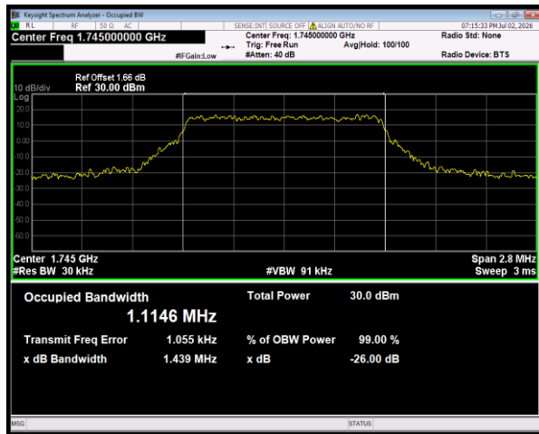
Band66 QPSK BW=1.4MHz Channel=132322 RB Size=6 Position=#0
