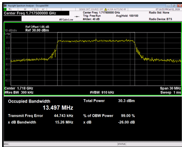
Band66 QPSK BW=15MHz Channel=132047 RB Size=75 Position=#0
