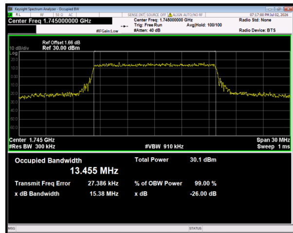
Band66 QPSK BW=15MHz Channel=132322 RB Size=75 Position=#0
