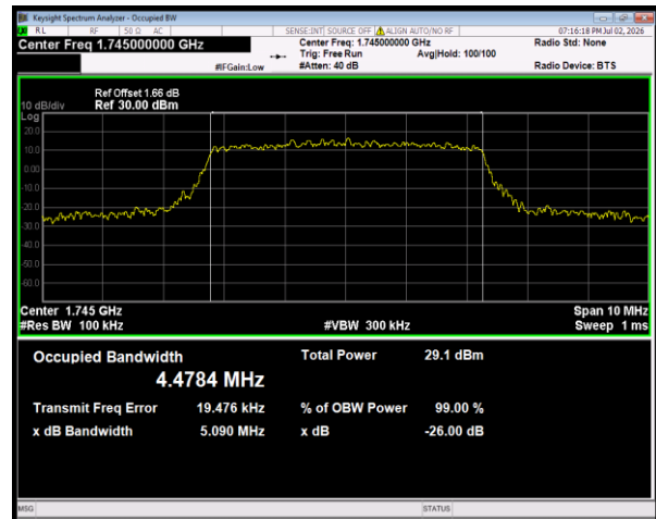
Band66 16QAM BW=5MHz Channel=132322 RB Size=25 Position=#0
