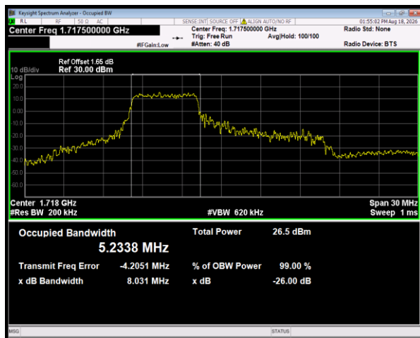
Band66 16QAM BW=15MHz Channel=132047 RB Size=27 Position=#0
