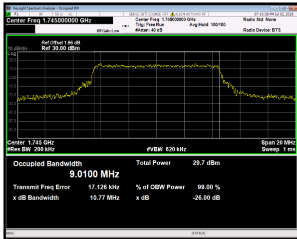
Band66 QPSK BW=10MHz Channel=132322 RB Size=50 Position=#0
