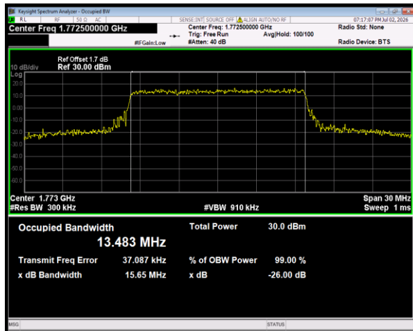
Band66 QPSK BW=15MHz Channel=132597 RB Size=75 Position=#0
