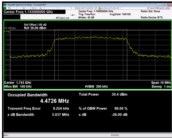
Band66 QPSK BW=5MHz Channel=132322 RB Size=25 Position=#0
