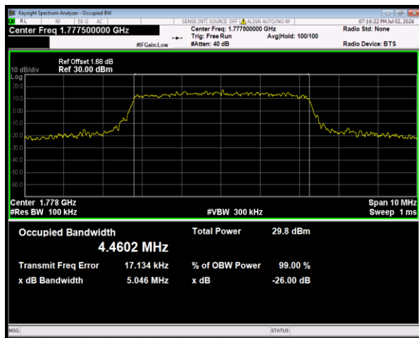
Band66 QPSK BW=5MHz Channel=132647 RB Size=25 Position=#0
