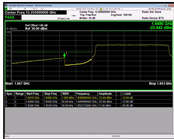
Band25 16QAM BW=3MHz LowChannel=26055 RB Size=15 Position=#0
