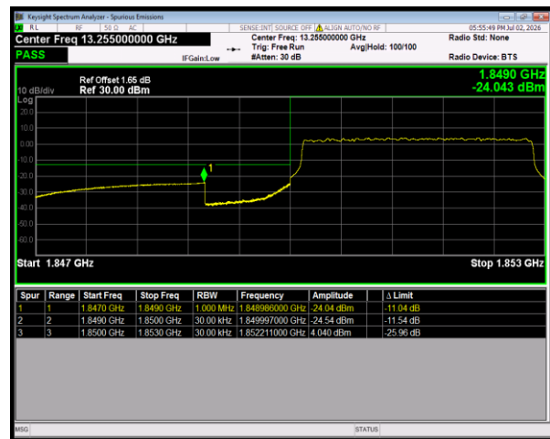
Band25 QPSK BW=3MHz LowChannel=26055 RB Size=15 Position=#0
