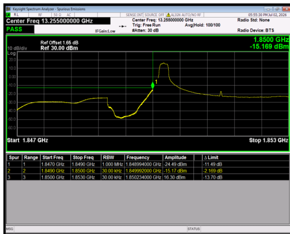
Band25 QPSK BW=3MHz LowChannel=26055 RB Size=1 Position=#0
