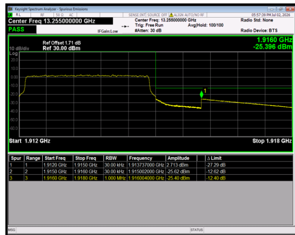
Band25 16QAM BW=3MHz HighChannel=26675 RB Size=15 Position=#0
