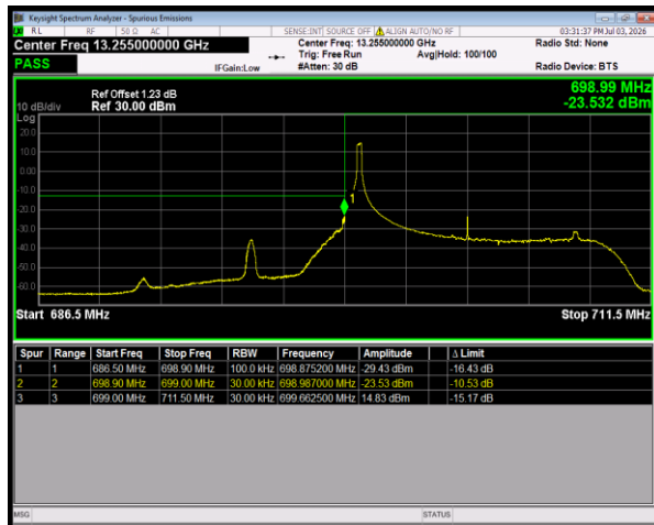
Band12 16QAM BW=10MHz LowChannel=23060 RB Size=1 Position=#0
