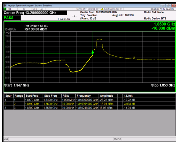
Band25 16QAM BW=3MHz LowChannel=26055 RB Size=1 Position=#0
