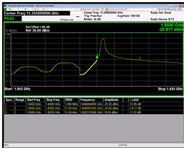
Band25 QPSK BW=5MHz LowChannel=26065 RB Size=1 Position=#0
