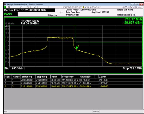
Band12 16QAM BW=10MHz HighChannel=23130 RB Size=27 Position=#Max
