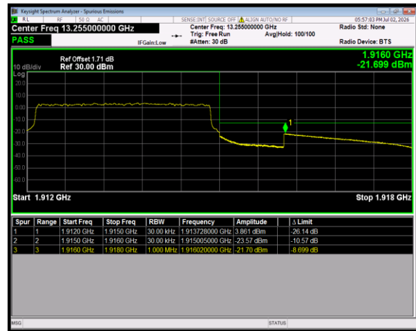
Band25 QPSK BW=3MHz HighChannel=26675 RB Size=15 Position=#0
