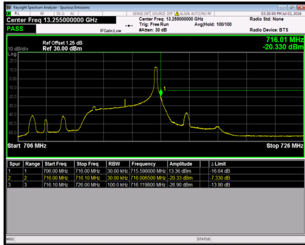
Band12 16QAM BW=5MHz HighChannel=23155 RB Size=1 Position=#Max
