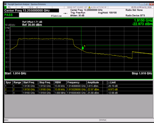
Band25 16QAM BW=1.4MHz HighChannel=26683 RB Size=6 Position=#0
