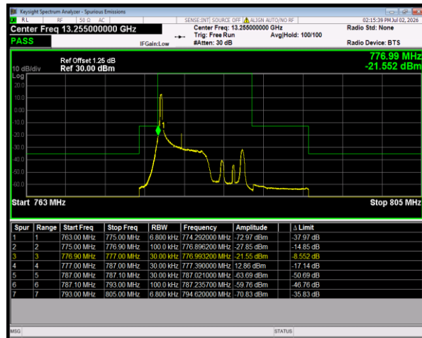
Band13 16QAM BW=5MHz LowChannel=23205 RB Size=1 Position=#0
