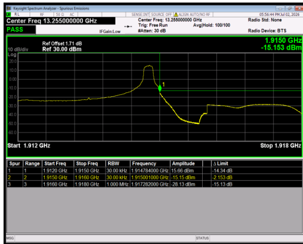
Band25 QPSK BW=3MHz HighChannel=26675 RB Size=1 Position=#Max
