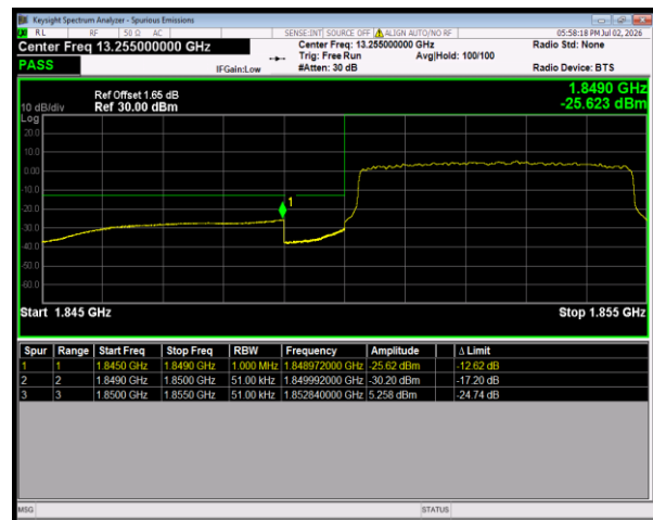
Band25 QPSK BW=5MHz LowChannel=26065 RB Size=25 Position=#0
