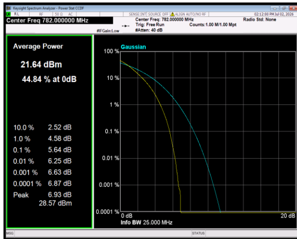
Band13 QPSK BW=10MHz Channel=23230 RB Size=50 Position=#0
