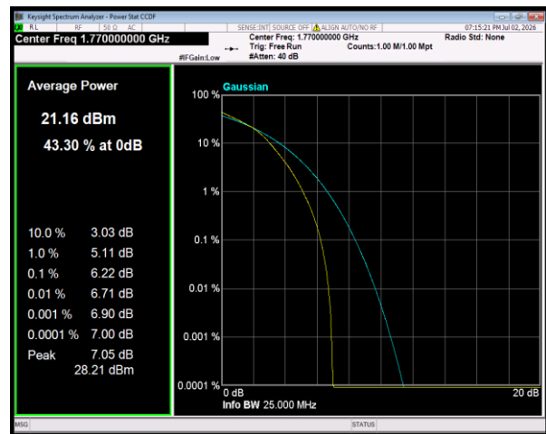
Band66 16QAM BW=20MHz Channel=132572 RB Size=27 Position=#0
