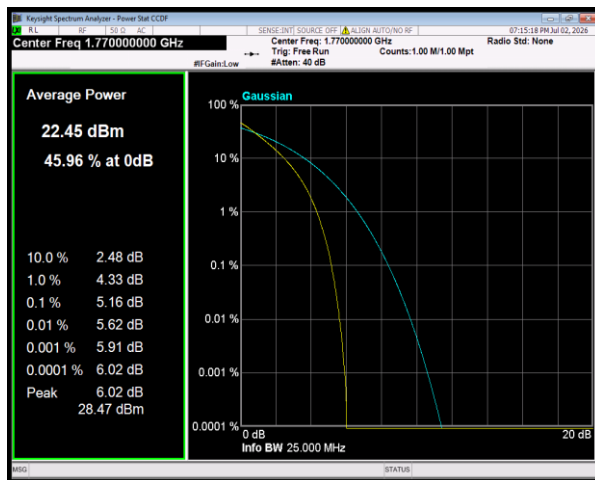
Band66 QPSK BW=20MHz Channel=132572 RB Size=100 Position=#0
