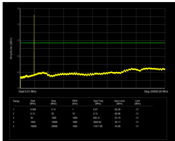
Band25 QPSK BW=5MHz Channel=26665 RB Size=1 Position=#0
