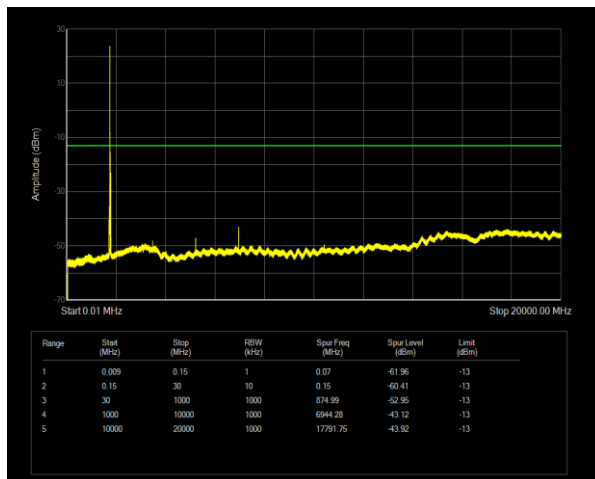
Band4 QPSK BW=20MHz Channel=20300 RB Size=1 Position=#0
