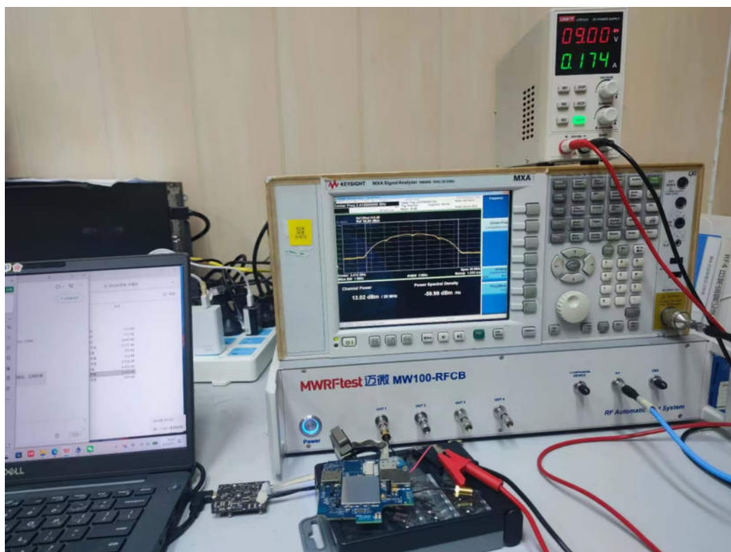
WLAN Test Setup
