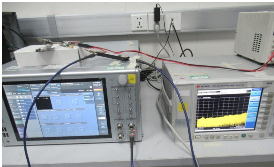
WWAN Test Setup
