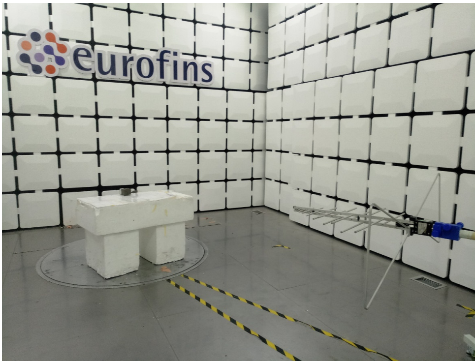
30MHz-1GHz
