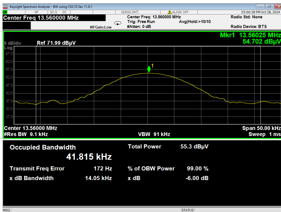
Figure 4 – Occupied Bandwidth
