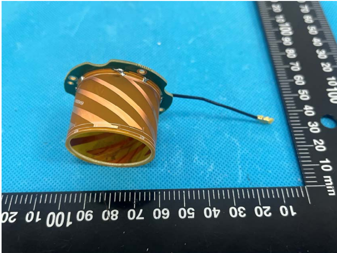
GNSS Antenna
