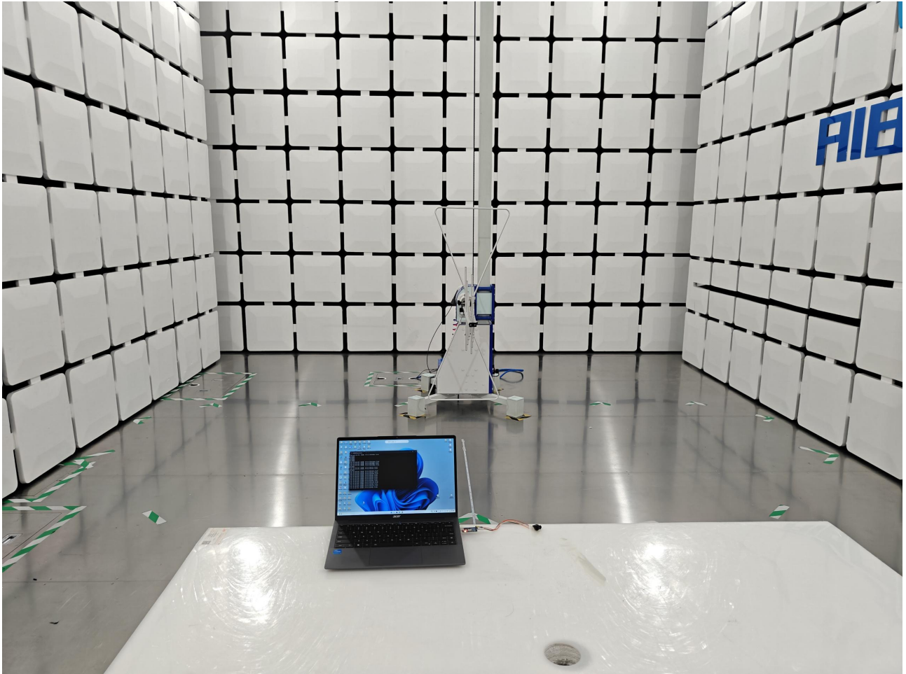
Radiated Spurious Emission Test View 1-left earphone
