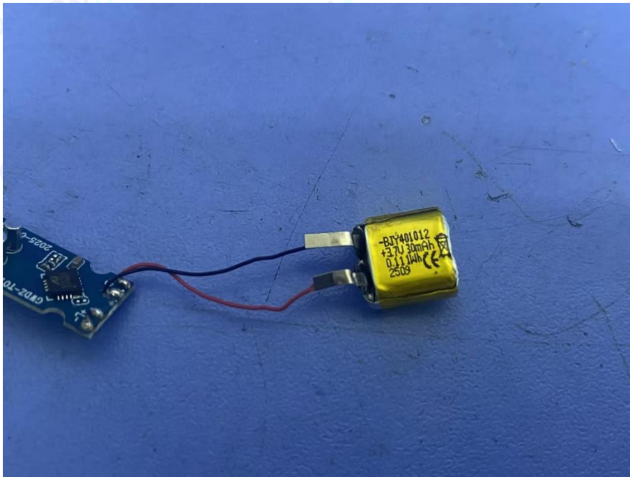
Photo 15 Internal of Battery
